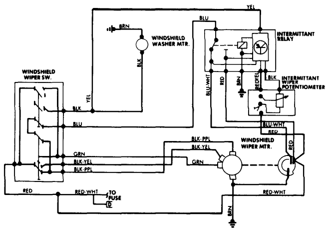
Windshield Wiper System Wiring Diagram (Peugeot 604)
