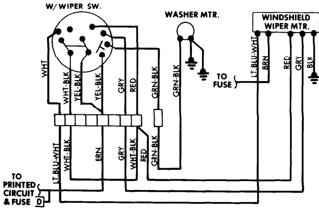
Windshield Wiper System Wiring Diagram (Fiat 128 Sedan)
