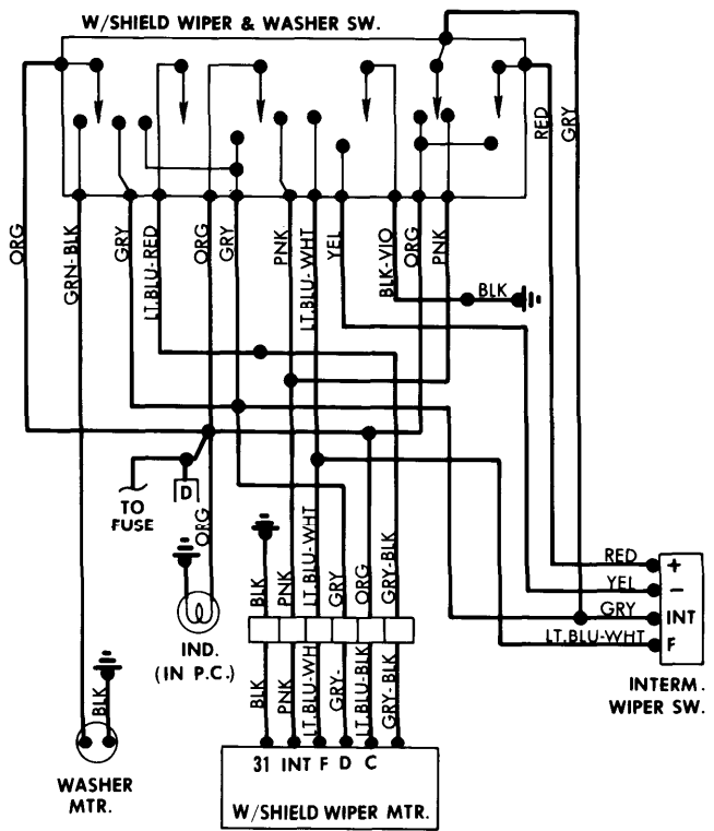
Windshield Wiper System Wiring Diagram (Fiat X1/9)
