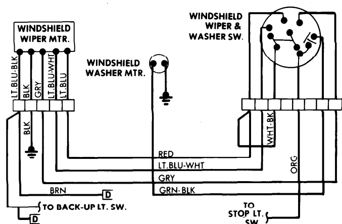
Windshield Wiper System Wiring Diagram (Fiat 128 3P)
