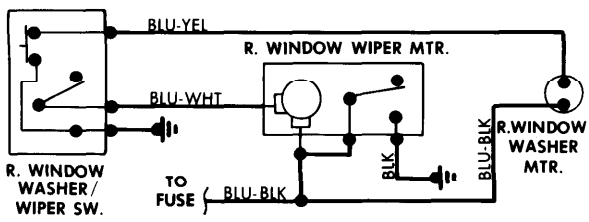
Windshield Wiper System Wiring Diagram (Mazda GLC)
