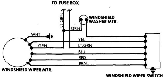
Windshield Wiper System Wiring Diagram (Jaguar)
