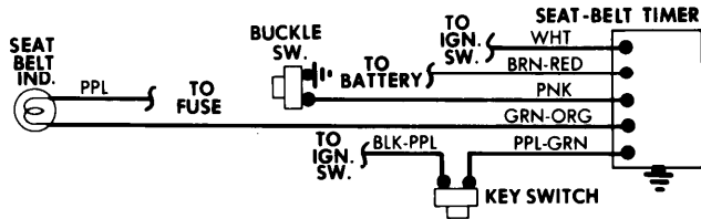
Seat Belt Warning System Wiring Diagram (Jaguar)
