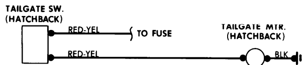
Tailgate Release System Wiring Diagram (Mazda GLC)
