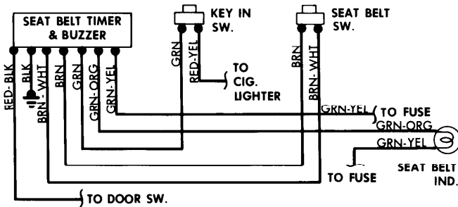
Seat Belt Warning System Wiring Diagram (Mazda)
