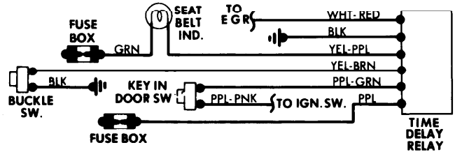
Seat Belt Warning System Wiring Diagram (MG Midget)
