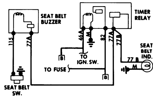
Seat Belt Warning System Wiring Diagram (Peugeot 604)
