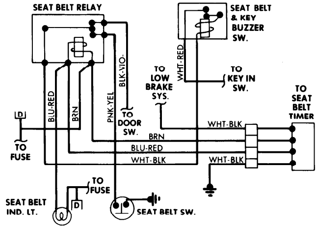
Seat Belt Warning System Wiring Diagram (Fiat 3P)
