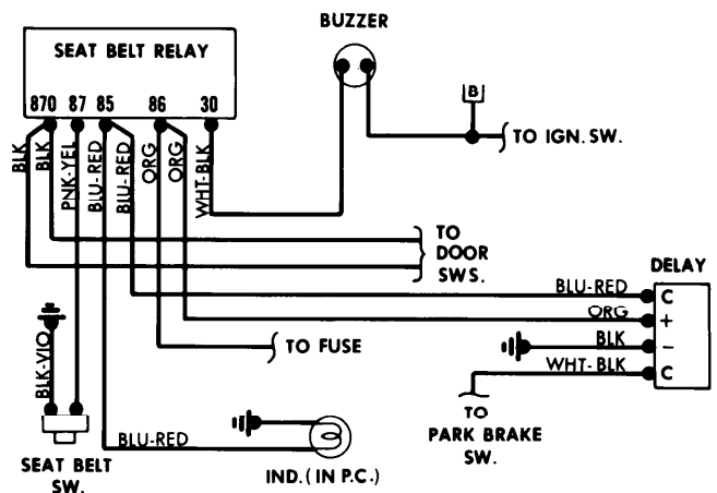
Seat Belt Warning System Wiring Diagram (Fiat X1/9)
