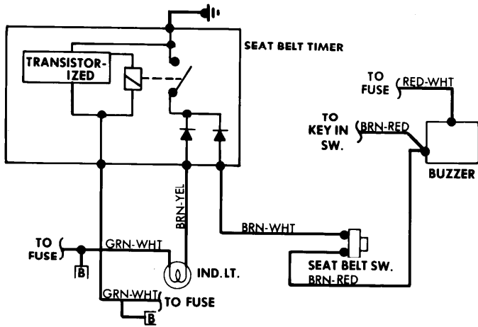
Seat Belt Warning System Wiring Diagram (BMW 633CSi)
