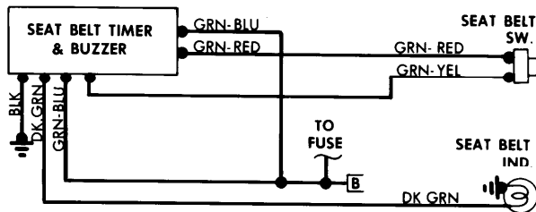
Seat Belt Warning System Wiring Diagram (Courier)
