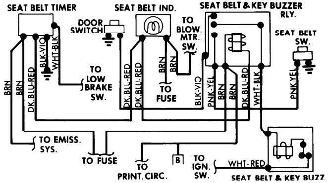
Seat Belt Warning System Wiring Diagram (Fiat 128)
