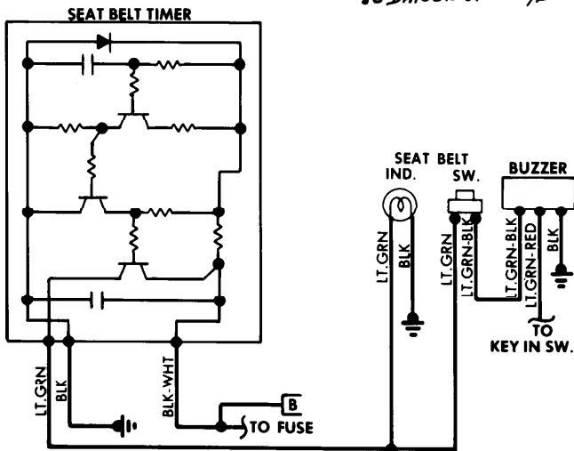
Seat Belt Warning System Wiring Diagram (Datsun 810)
