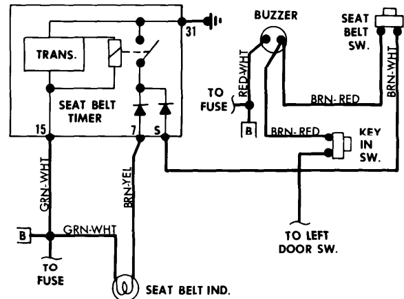
Seat Belt Warning System Wiring Diagram (BMW 320i)
