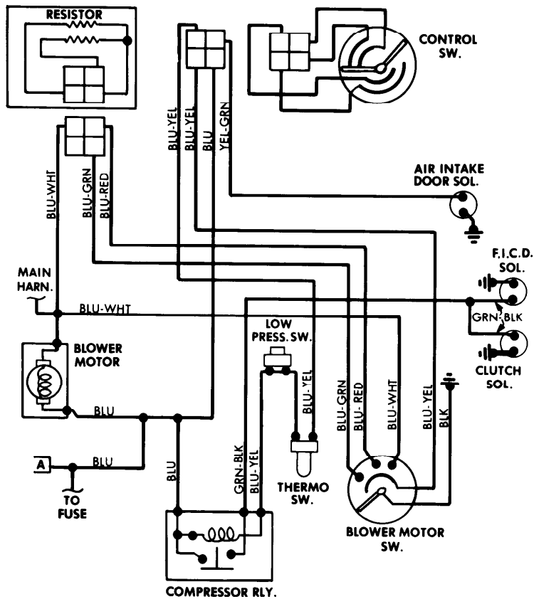
Heater and Air Conditioning System (Datsun 810)
