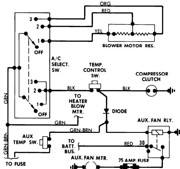
Heater and Air Conditioning System (BMW 320i)
