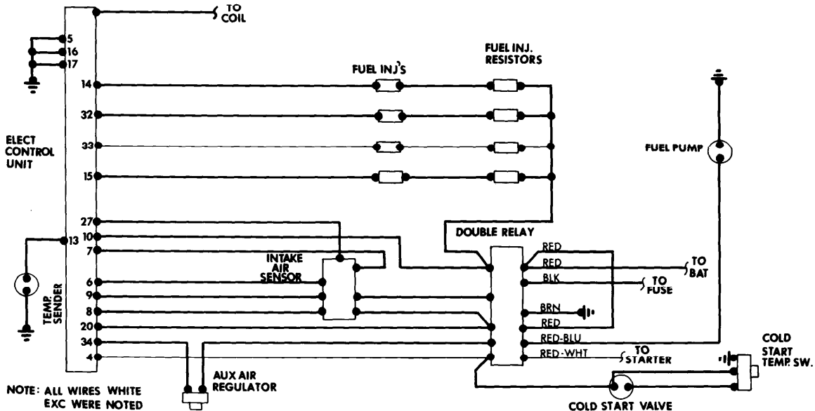
Fuel Injection System Wiring Diagram (Volkswagen Type 1)
