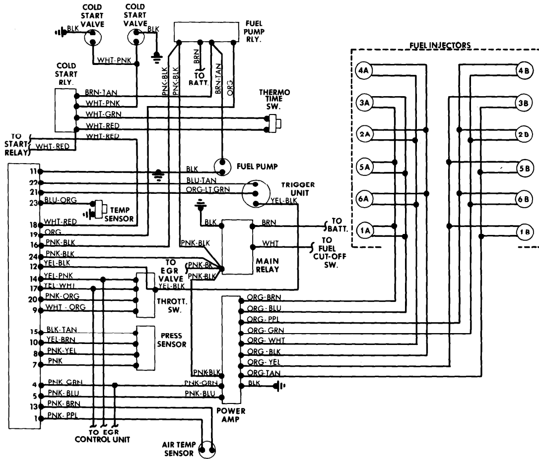
Fuel Injection System Wiring Diagram (Jaguar XJ12 and XJS)
