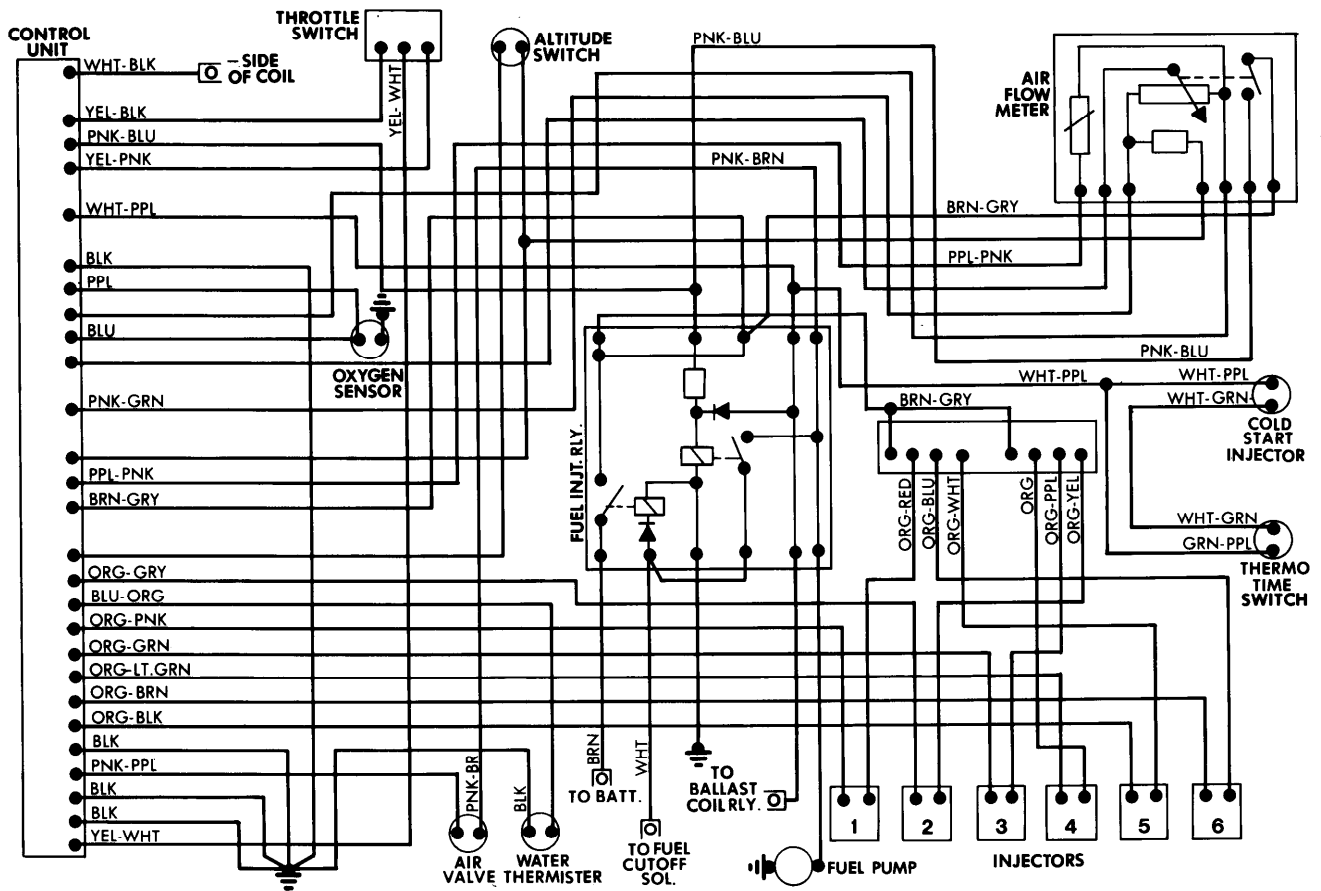
Fuel Injection System Wiring Diagram (Jaguar XJ6)
