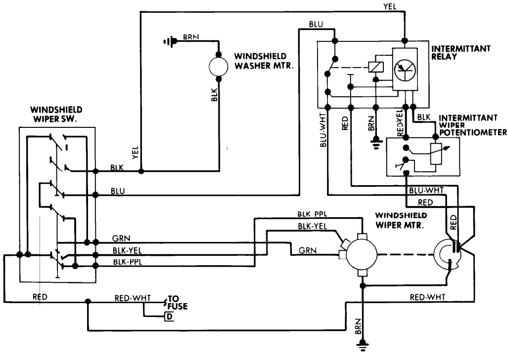
Windshield Wiper System Wiring Diagram (Porsche 911SC and Turbo)
