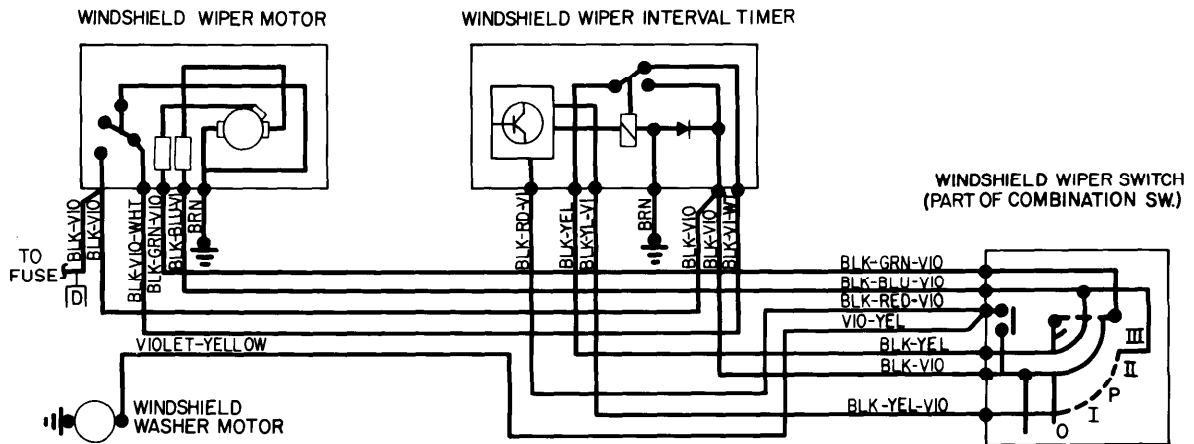
Windshield Wiper System Wiring Diagram (Mercedes Benz 230, 240D, 280, 280CE, 300D and 300CD)
