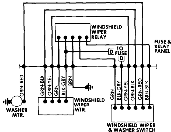
Windshield Wiper System Wiring Diagram (Porsche 924)
