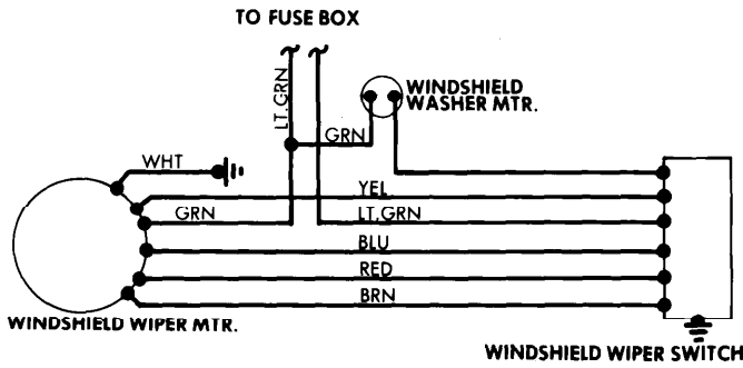
Windshield Wiper System Wiring Diagram (Jaguar)
