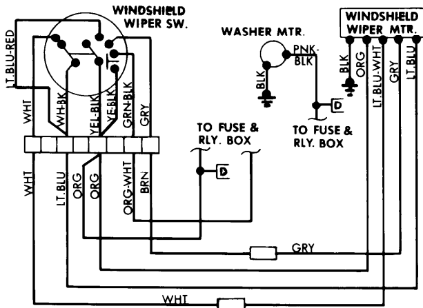
Windshield Wiper System Wiring Diagram (Fiat 131)
