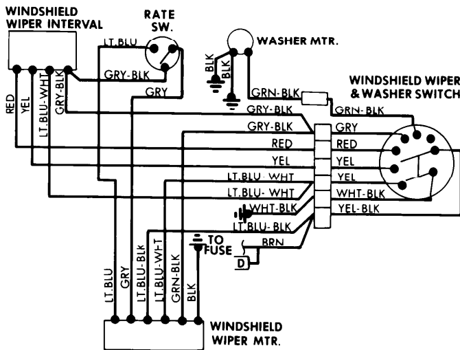
Windshield Wiper System Wiring Diagram (Fiat 124)
