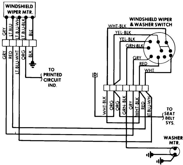
Windshield Wiper System Wiring Diagram (Fiat X1/9)
