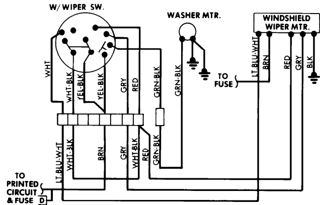
Windshield Wiper System Wiring Diagram (Fiat 128 Sedan)
