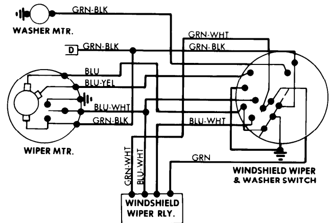
Windshield Wiper System Wiring Diagram (Honda Accord)
