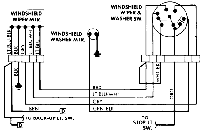
Windshield Wiper System Wiring Diagram (Fiat 128 3P)
