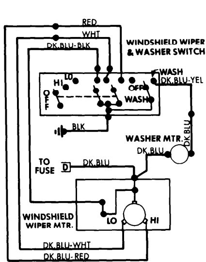
Windshield Wiper System Wiring Diagram (Courier)
