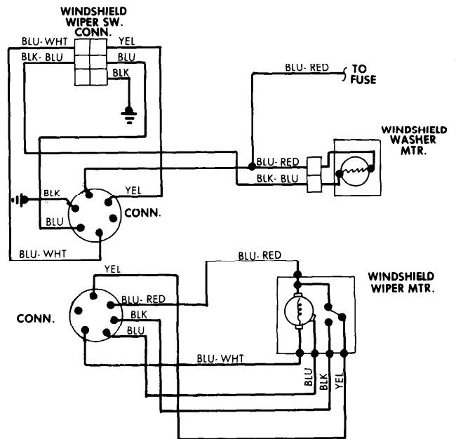
Windshield Wiper System Wiring Diagram (Datsun 510)
