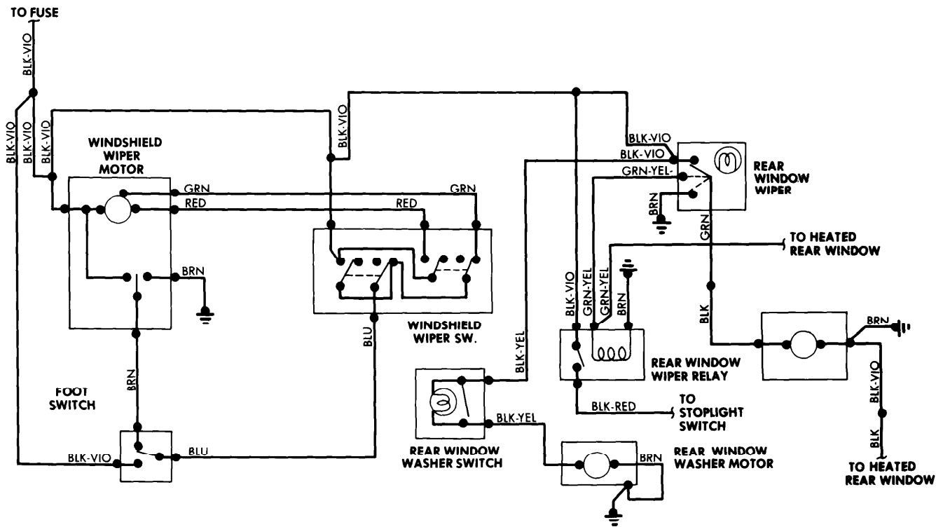
Windshield Wiper System Wiring Diagram (Capri)
