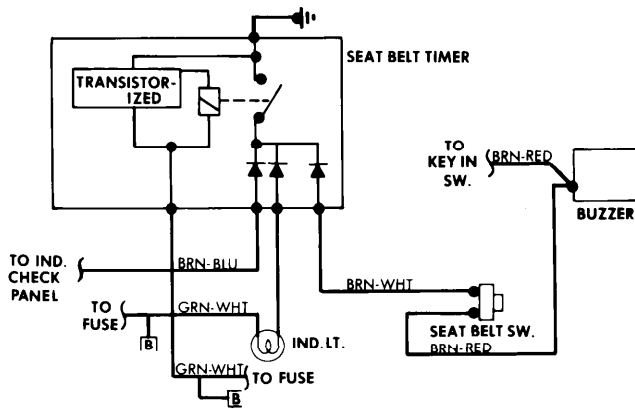
Seat Belt Warning System Wiring Diagram (BMW 633CSi and 733i)
