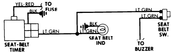
Seat Belt Warning System Wiring Diagram (Datsun F10)
