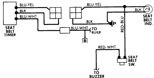
Seat Belt Warning System Wiring Diagram (Datsun 200SX)
