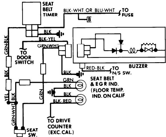
Seat Belt Warning System Wiring Diagram (Datsun B210)
