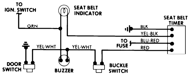
Seat Belt Warning System Wiring Diagram (Colt and Arrow)
