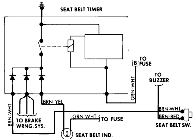
Seat Belt Warning System Wiring Diagram (BMW 320i)
