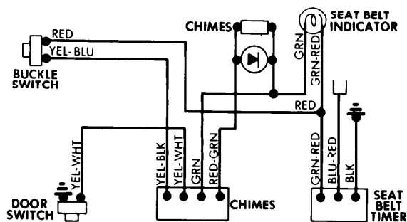
Seat Belt Warning System Wiring Diagram (Colt Station Wagon)
