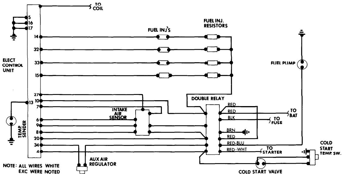
Fuel Injection System Wiring Diagram (Volkswagen Type 1 & 2)
