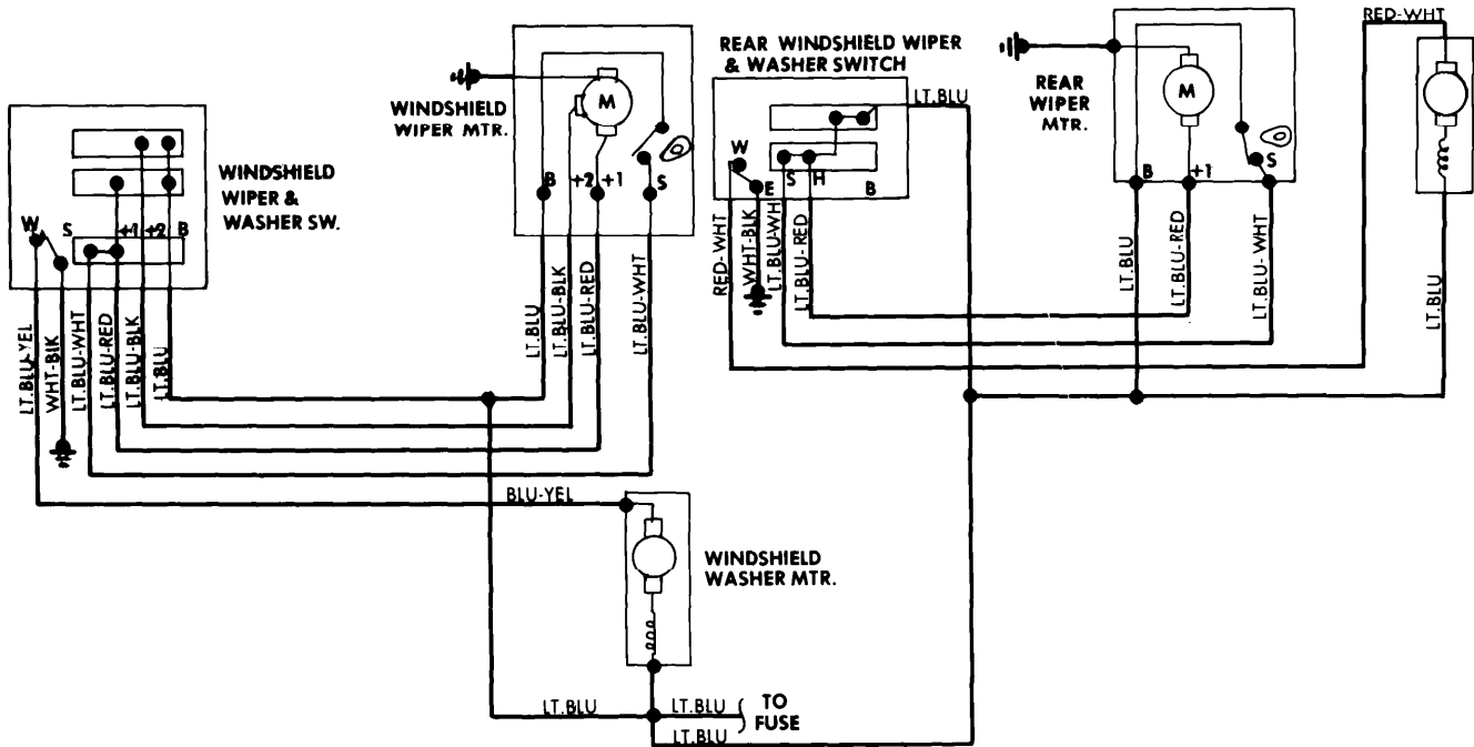
Windshield Wiper System Wiring Diagram (Toyota Corona)
