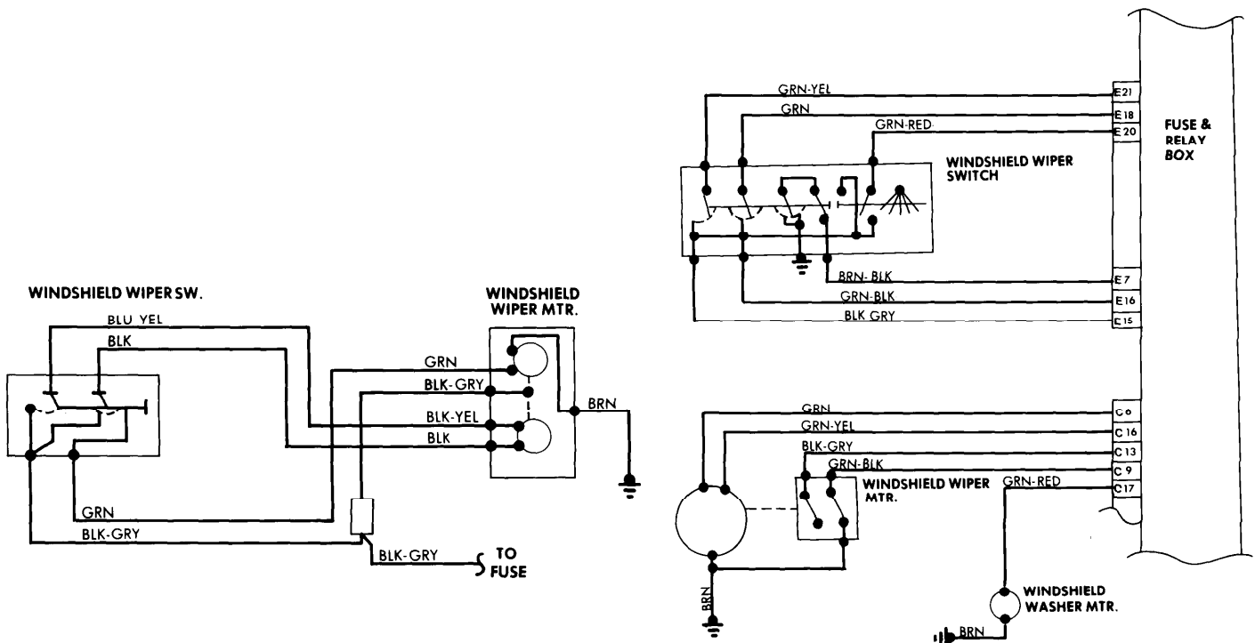
Windshield Wiper System Wiring Diagram (Volkswagen Type 1 and 2)
