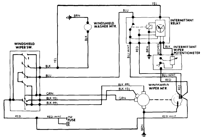
Windshield Wiper System Wiring Diagram (Peugeot 604)
