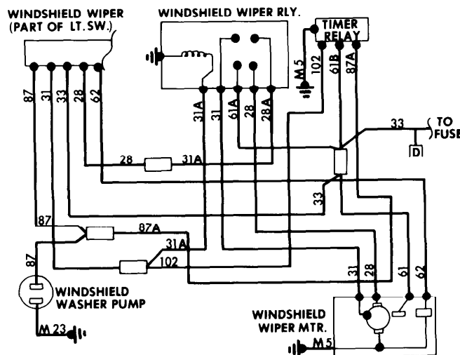
Windshield Wiper System Wiring Diagram (911S and Turbo Carrera)
