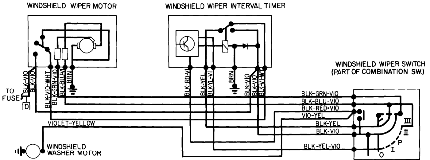
Windshield Wiper System Wiring Diagram (Mercedes-Benz 240D, 280E and 300D)
