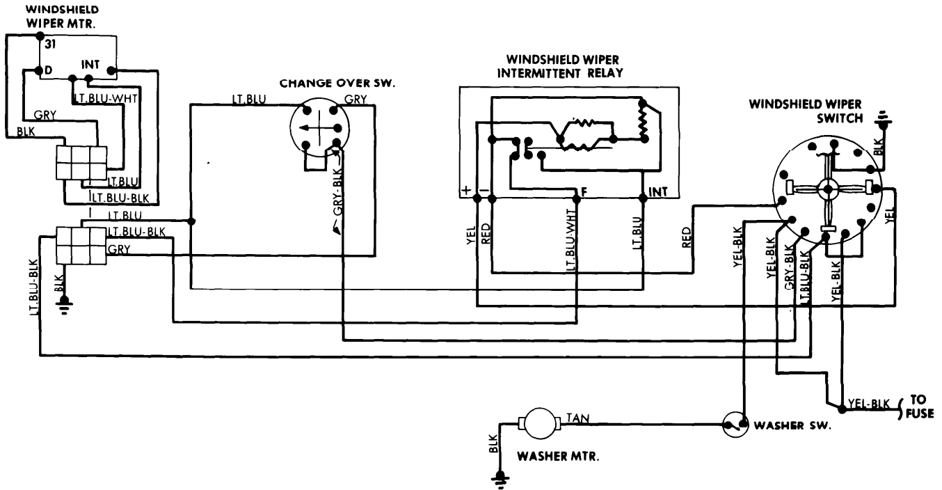
Windshield Wiper System Wiring Diagram (Lancia)
