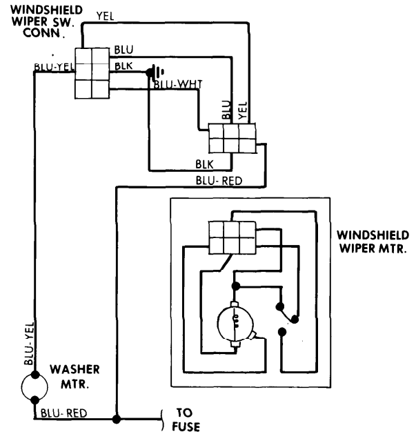
Windshield Wiper System Wiring Diagram (Datsun F10)
