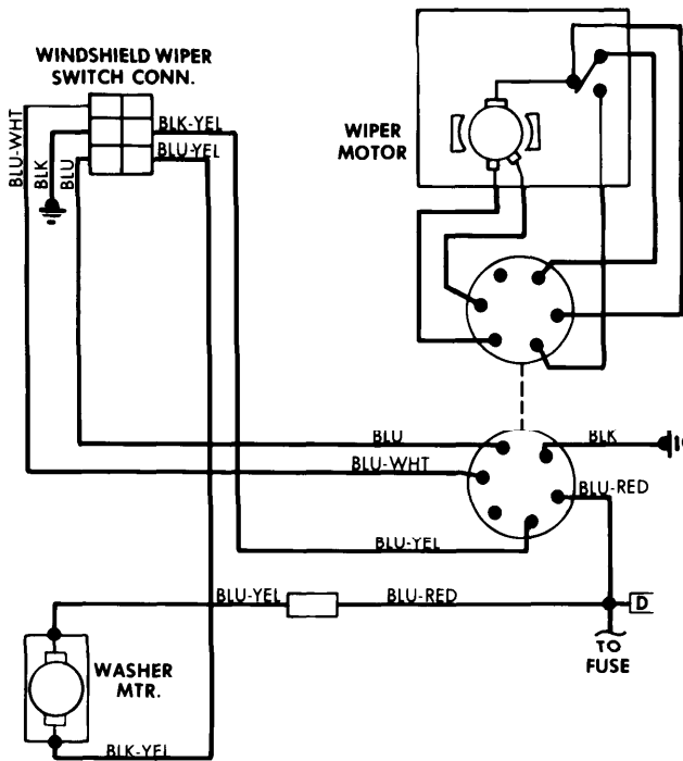
Windshield Wiper System Wiring Diagram (Datsun B210)
