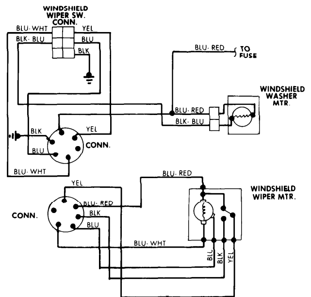
Windshield Wiper System Wiring Diagram (Datsun 710)
