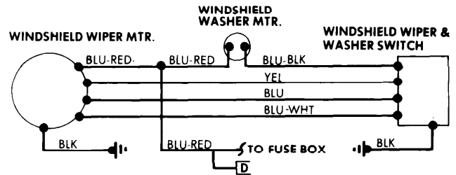
Windshield Wiper System Wiring Diagram (Datsun Pickup)
