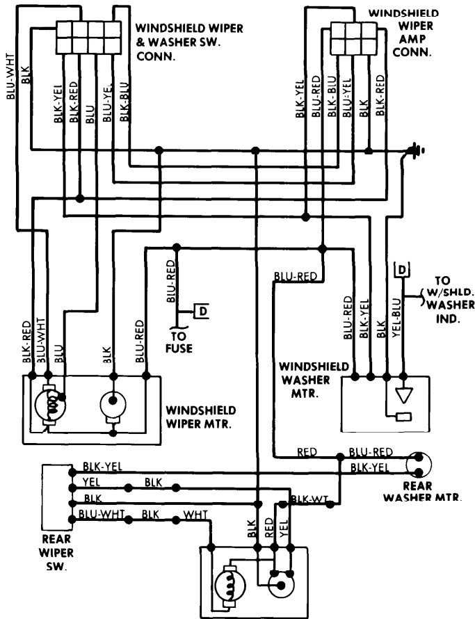
Windshield Wiper System Wiring Diagram (Datsun 810)
