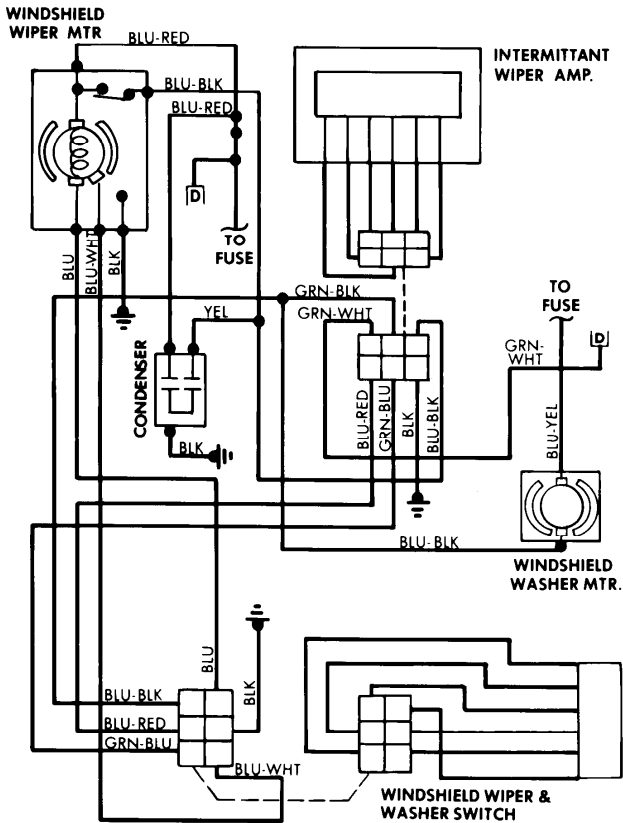
Windshield Wiper System Wiring Diagram (Capri)
