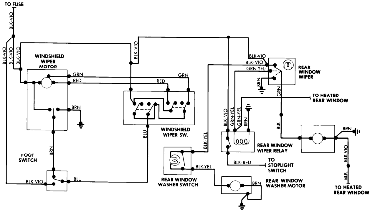
Windshield Wiper System Wiring Diagram (Capri)
