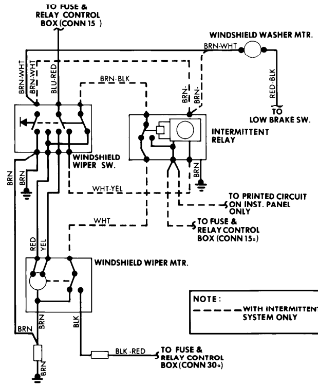
Windshield Wiper System Wiring Diagram (Audi 100LS)
