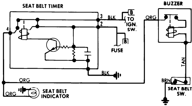
Seat Belt Warning System Wiring Diagram (Renault Gordini)
