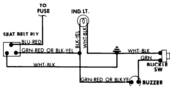
Seat Belt Warning System Wiring Diagram (Toyota Celica and Land Cruiser FJ40)
