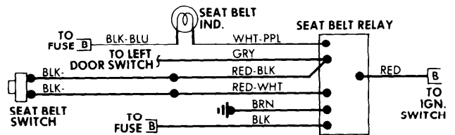
Seat Belt Warning System Wiring Diagram (Porsche 924)
