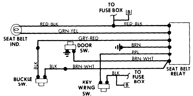
Seat Belt Warning System Wiring Diagram (Porsche 911 & 930)
