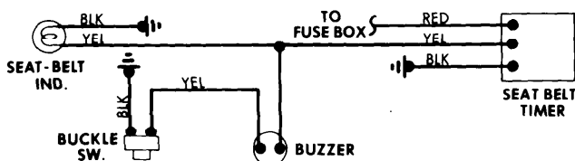
Seat Belt Warning System Wiring Diagram (Opel)
