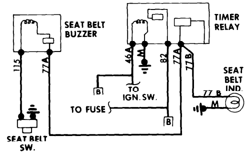
Seat Belt Warning System Wiring Diagram (Peugeot 604)
