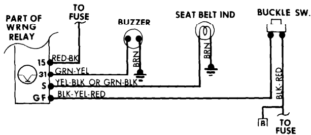
Seat Belt Warning System Wiring Diagram (Mercedes 450SEL, 450SL-SLC and 6.9)
