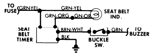
Seat Belt Warning System Wiring Diagram (Mazda RX3SP and GLC)
