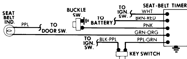
Seat Belt Warning System Wiring Diagram (Honda)
