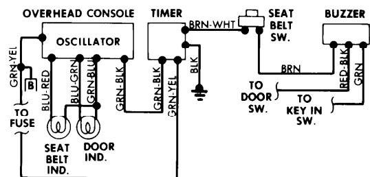
Seat Belt Warning System Wiring Diagram (Mazda RX4)
