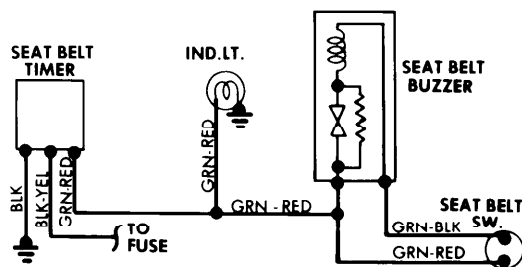
Seat Belt Warning System Wiring Diagram (LUV)
