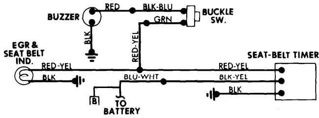
Seat Belt Warning System Wiring Diagram (Datsun 620 Pickup)
