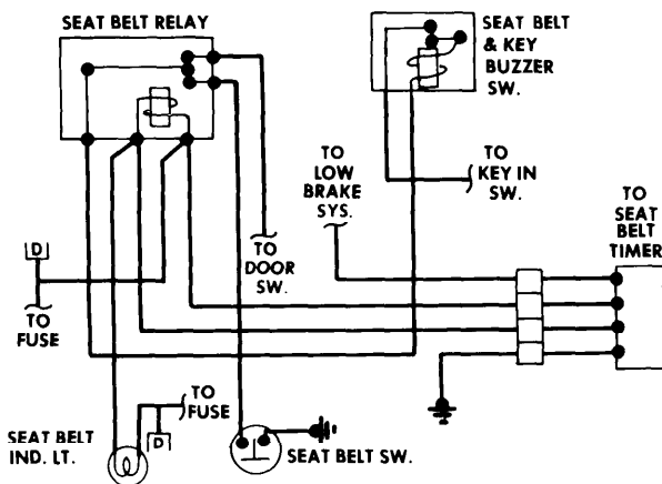
Seat Belt Warning System Wiring Diagram (Fiat 3P)
