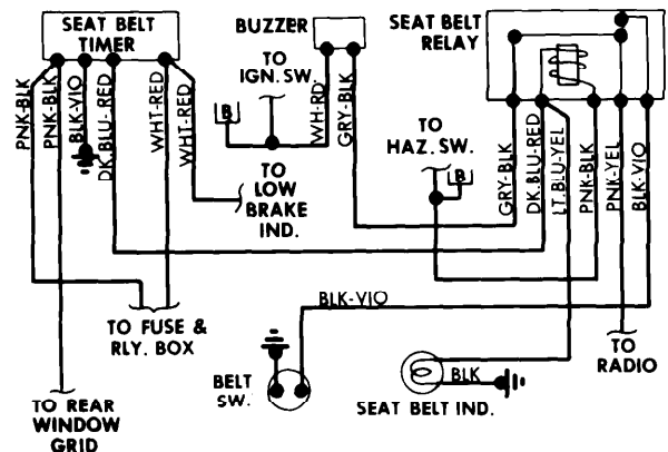
Seat Belt Warning System Wiring Diagram (Fiat 131)
