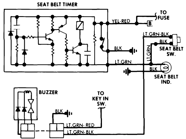
Seat Belt Warning System Wiring Diagram (Datsun 710)
