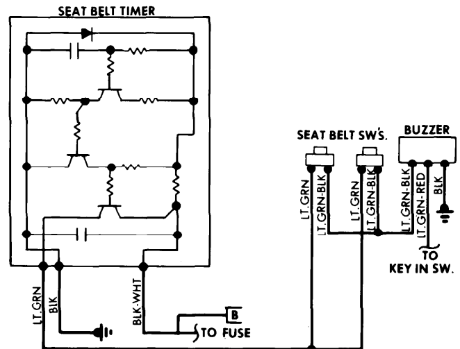
Seat Belt Warning System Wiring Diagram (Datsun 810)
