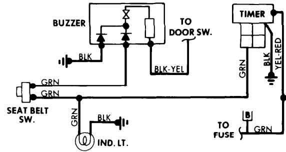
Seat Belt Warning System Wiring Diagram (Datsun 280Z)
