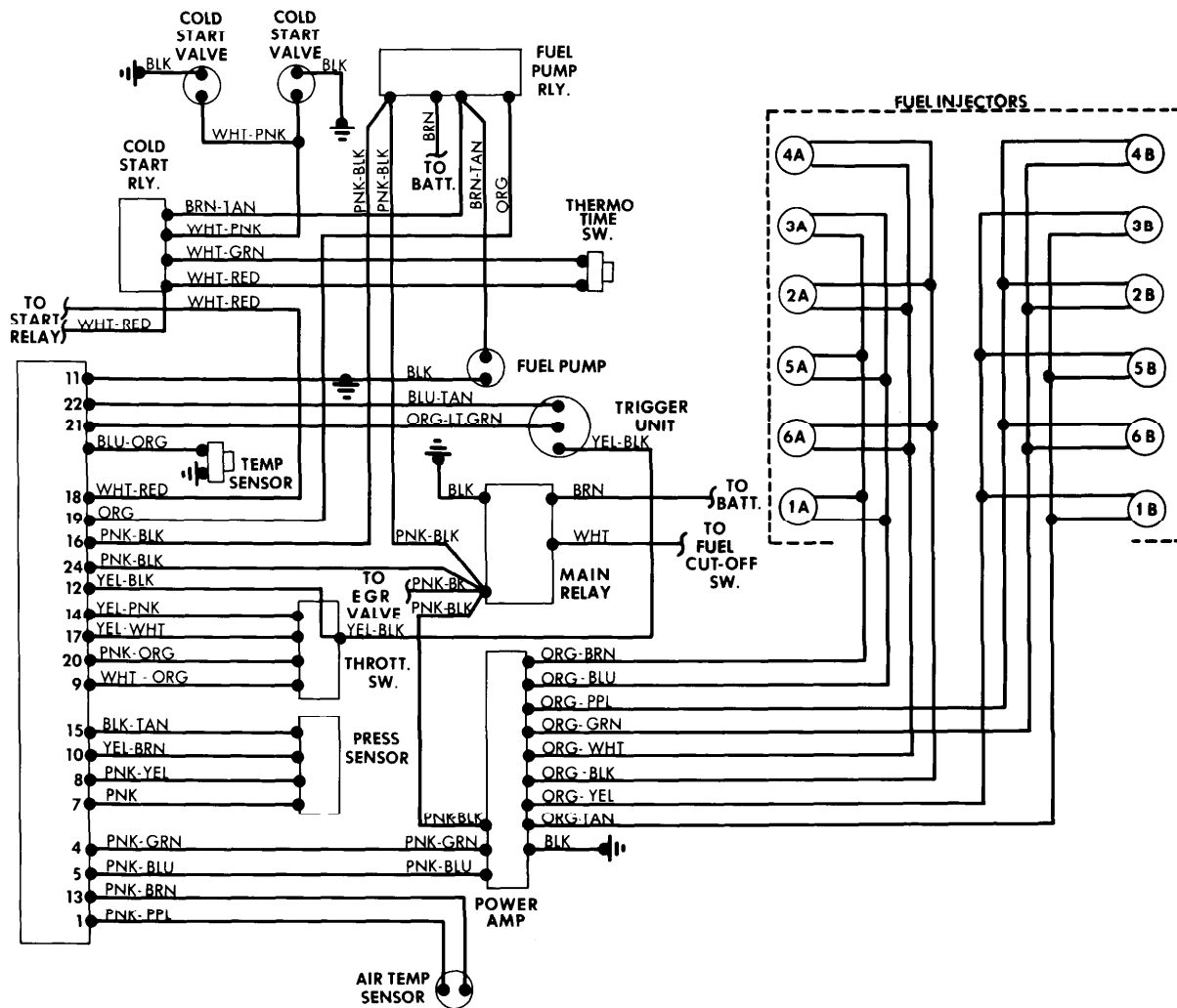
Fuel Injection System Wiring Diagram (Jaguar V12)
