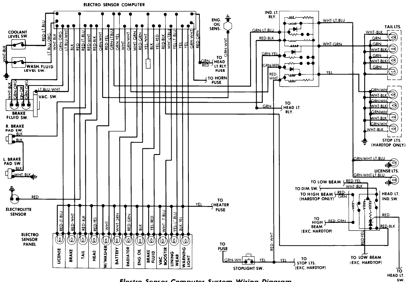
Electro Sensor Computer System Wiring Diagram (Toyota, All Models So Equipped)
