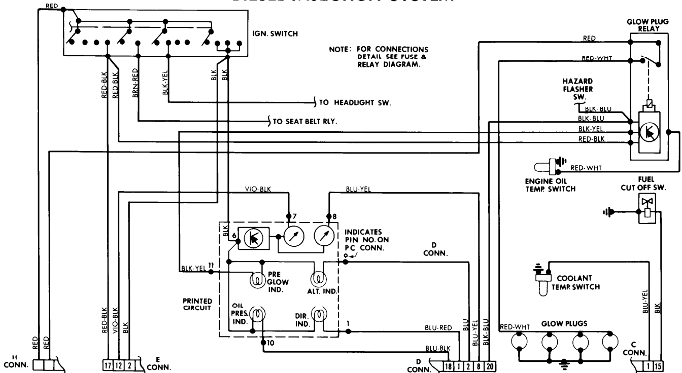
Diesel Injection System Wiring Diagram (Volkswagen Rabbit Diesel)
