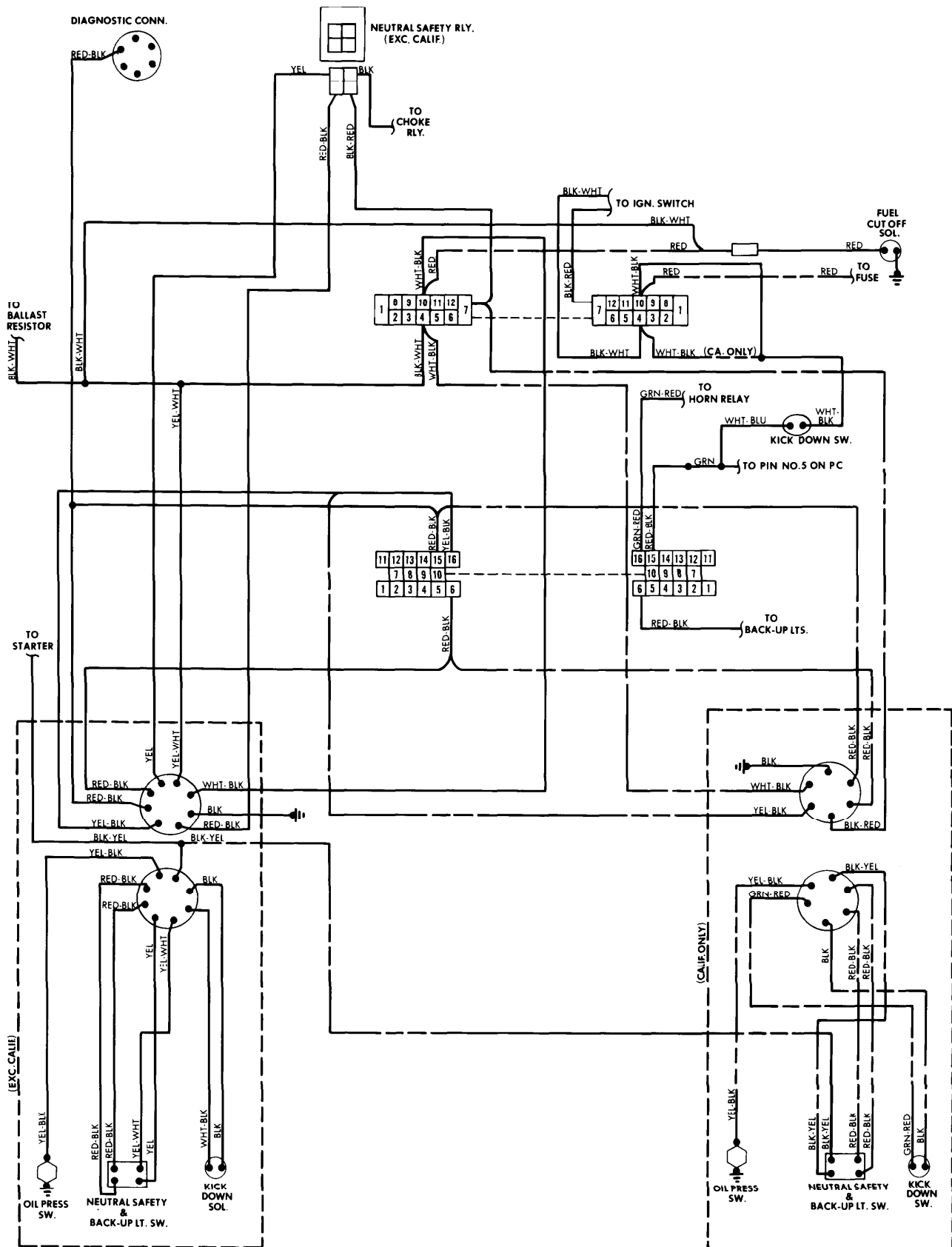
Automatic Transmission System (Datsun 200SX)
