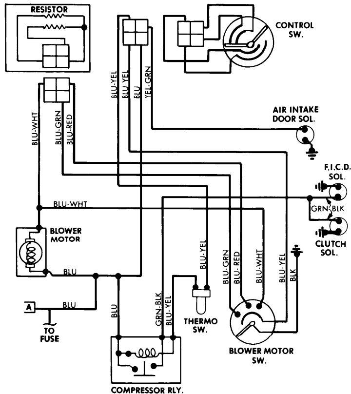
Heater and Air Conditioning System (Datsun 810)
