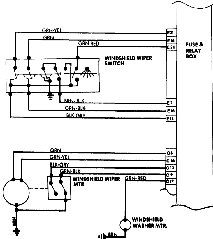
Windshield Wiper System Wiring Diagram (Volkswagen Rabbit and Scirocco)
