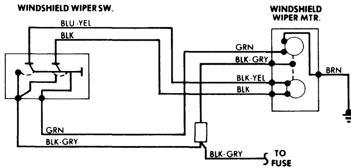
Windshield Wiper System Wiring Diagram (Volkswagen Type 1 and Type 2)
