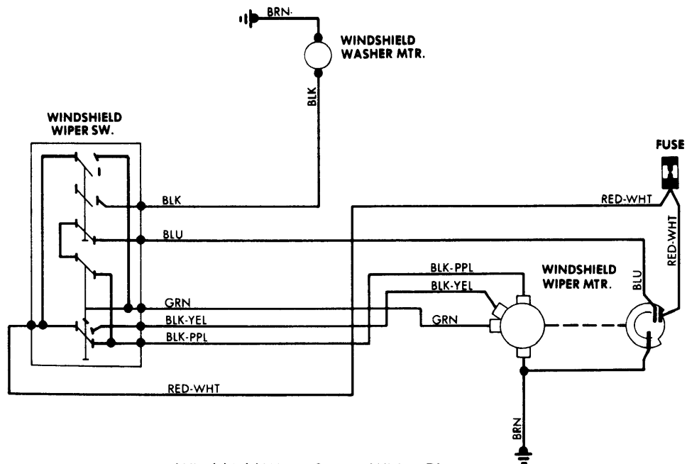
Windshield Wiper System Wiring Diagram (Porsche 911S)
