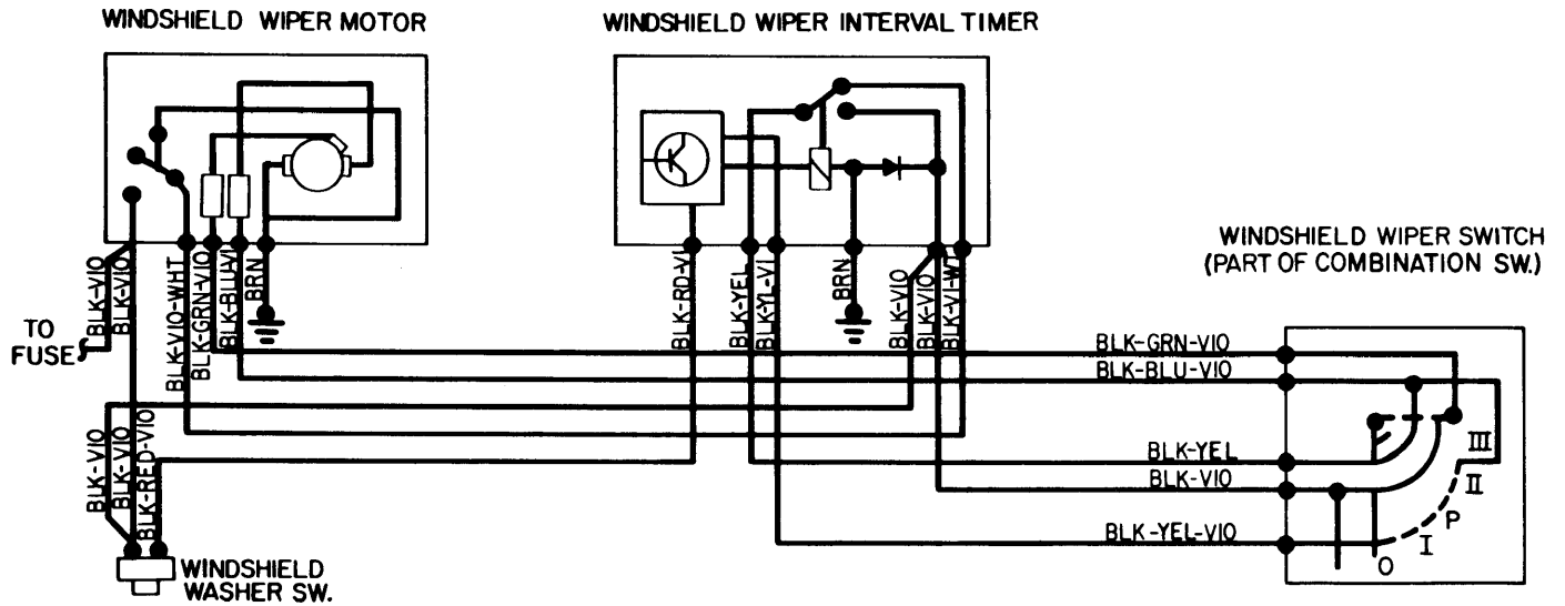
Windshield Wiper System Wiring Diagram (Mercedes-Benz 230)
