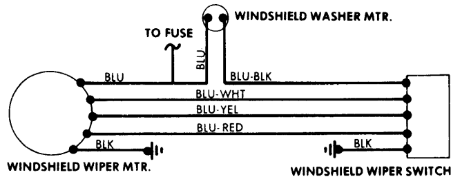
Windshield Wiper System Wiring Diagram (Opel)
