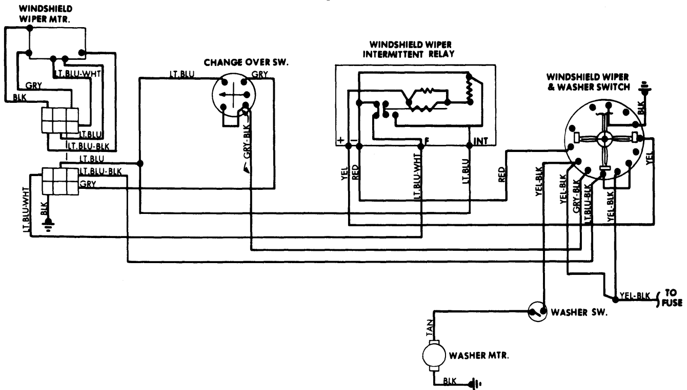
Windshield Wiper System Wiring Diagram (Lancia)
