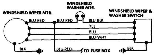
Windshield Wiper System Wiring Diagram (Datsun Pickup)
