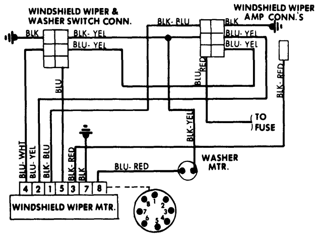
Windshield Wiper System Wiring Diagram (Datsun 610)
