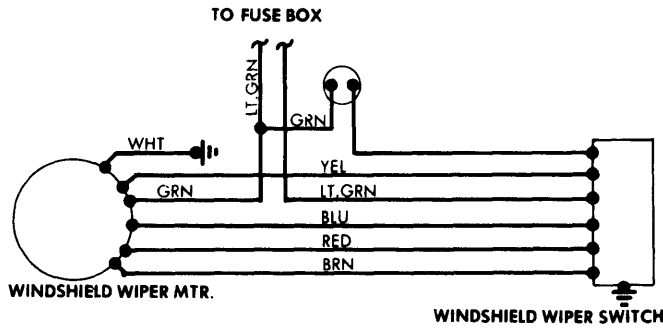
Windshield Wiper System Wiring Diagram (Jaguar XJS)
