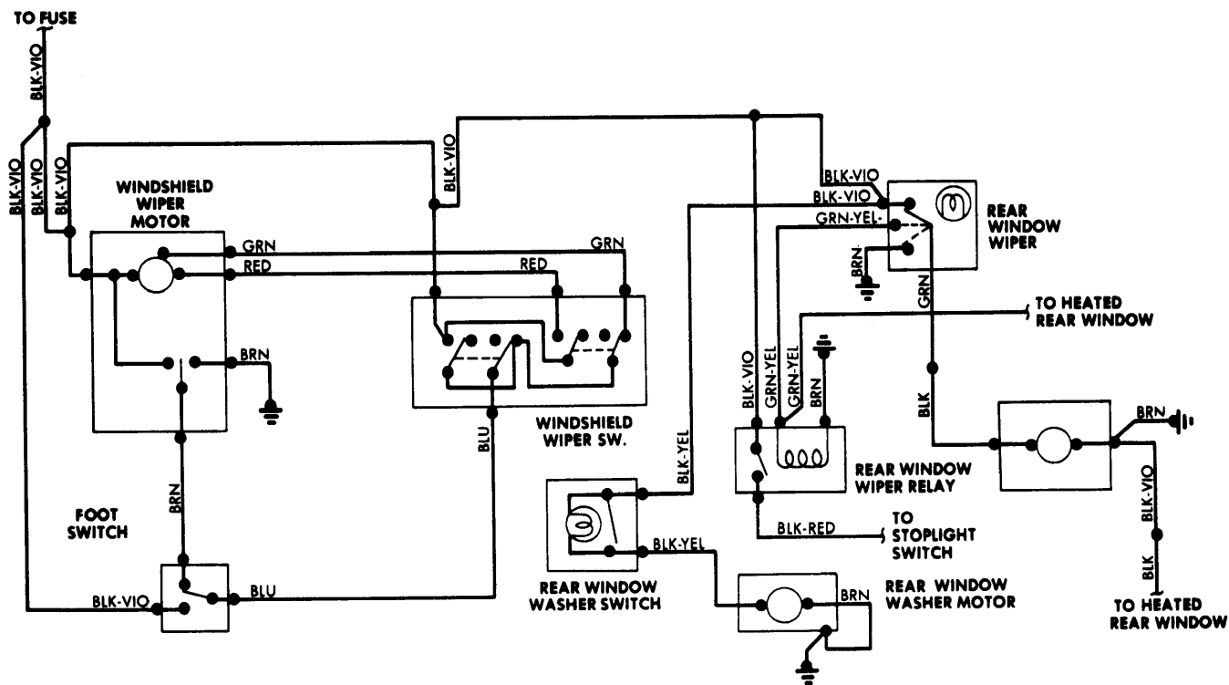
Windshield Wiper System Wiring Diagram (Capri II)
