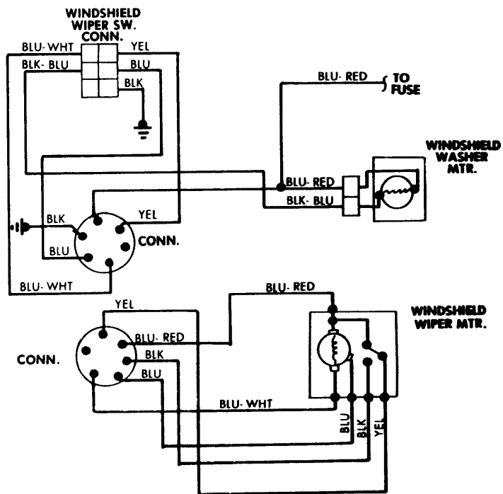
Windshield Wiper System Wiring Diagram (Datsun B210)
