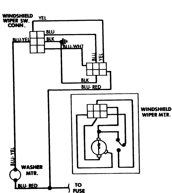
Windshield Wiper System Wiring Diagram (Datsun F10)
