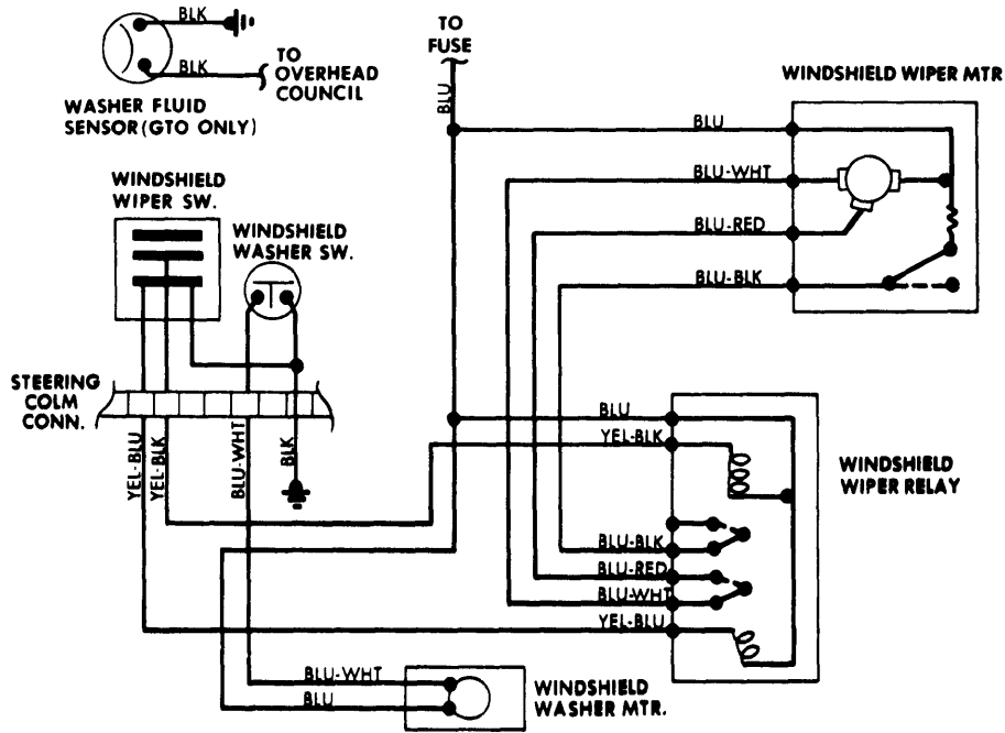
Windshield Wiper System Wiring Diagram (Arrow and Colt)
