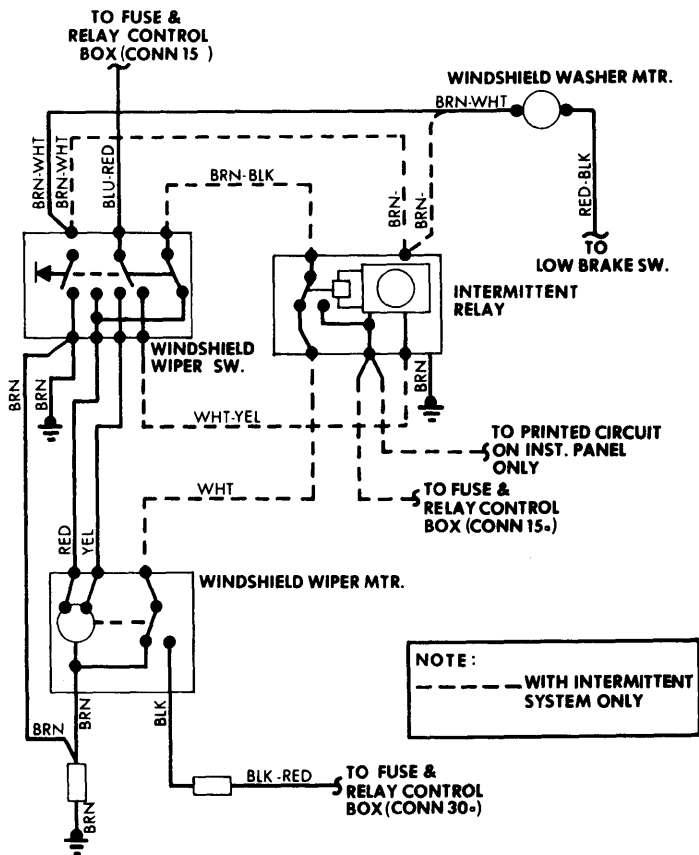
Windshield Wiper System Wiring Diagram (Audi 100LS)
