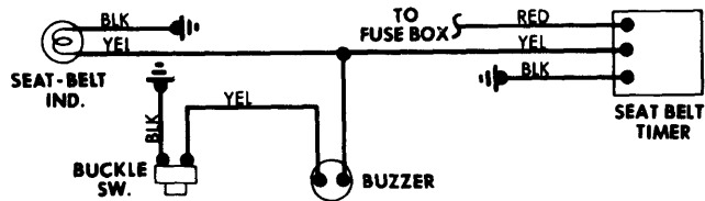
Seat Belt Warning System Wiring Diagram (Opel)
