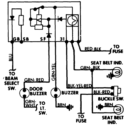
Seat Belt Warning System Wiring Diagram (Mercedes-Benz 280S)
