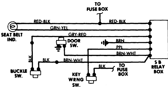
Seat Belt Warning System Wiring Diagram (Porsche 911S, 912E and Turbo Carrera)
