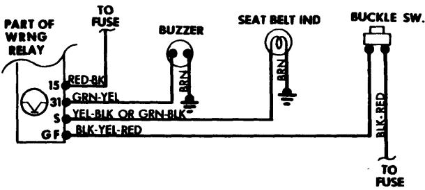
Seat Belt Warning System Wiring Diagram (Mercedes-Benz All Models Except 280S)
