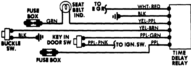
Seat Belt Warning System Wiring Diagram (MG Midget and MGB)
