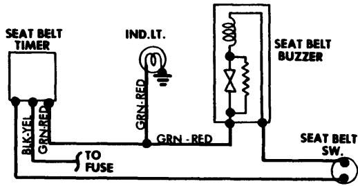
Seat Belt Warning System Wiring Diagram (LUV)
