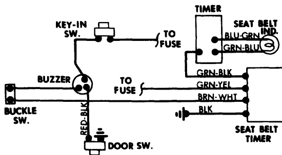
Seat Belt Warning System Wiring Diagram (Mazda RX4)
