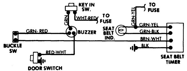
Seat Belt Warning System Wiring Diagram (Mazda Cosmo)
