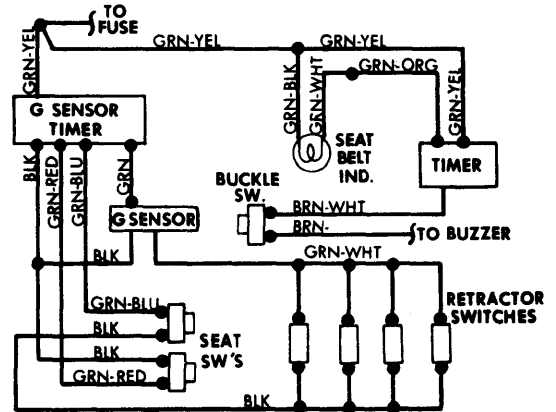
Seat Belt Warning System Wiring Diagram (Mazda 808)
