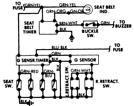
Seat Belt Warning System Wiring Diagram (Mazda RX3)
