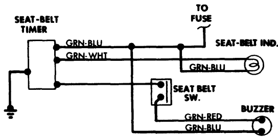
Seat Belt Warning System Wiring Diagram (Mazda B1600)
