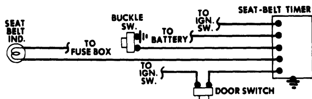
Seat Belt Warning System Wiring Diagram (Jaguar XJS)
