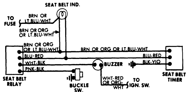
Seat Belt Warning System Wiring Diagram (Fiat 124, 128 and X1/9)
