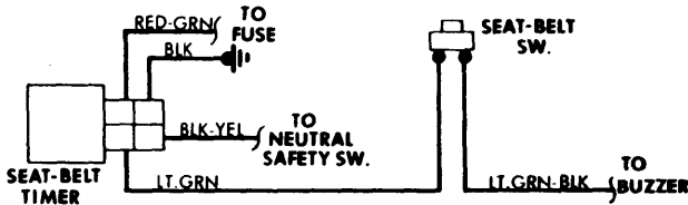
Seat Belt Warning System Wiring Diagram (Datsun 610)
