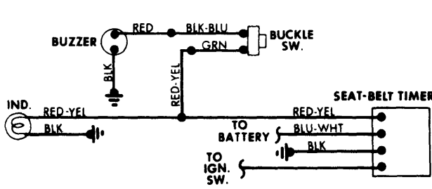
Seat Belt Warning System Wiring Diagram (Datsun Pickup)
