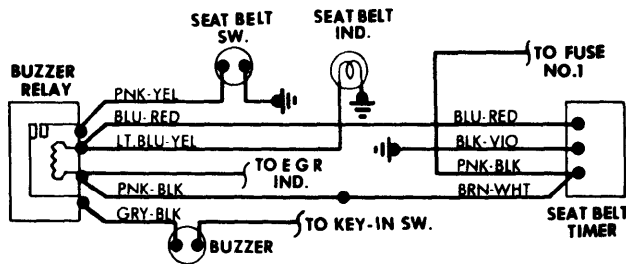
Seat Belt Warning System Wiring Diagram (Fiat 131)
