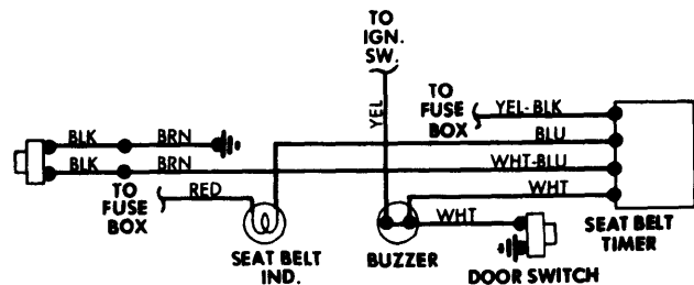
Seat Belt Warning System Wiring Diagram (Lancia)
