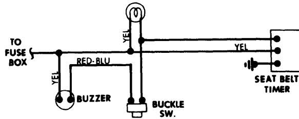
Seat Belt Warning System Wiring Diagram (Honda)
