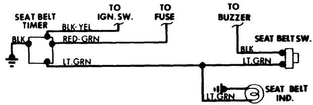
Seat Belt Warning System Wiring Diagram (Datsun 710)
