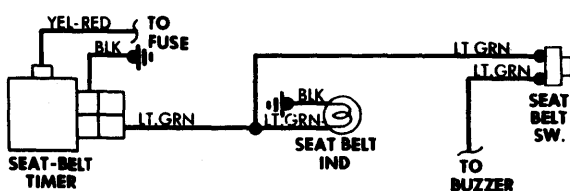
Seat Belt Warning System Wiring Diagram (Datsun F10)
