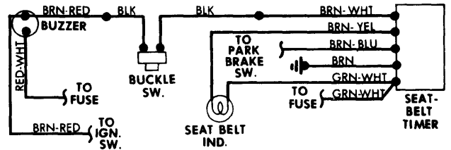
Seat Belt Warning System Wiring Diagram (BMW 2002 and 3.0Si)
