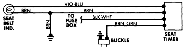
Seat Belt Warning System Wiring Diagram (Capri II)
