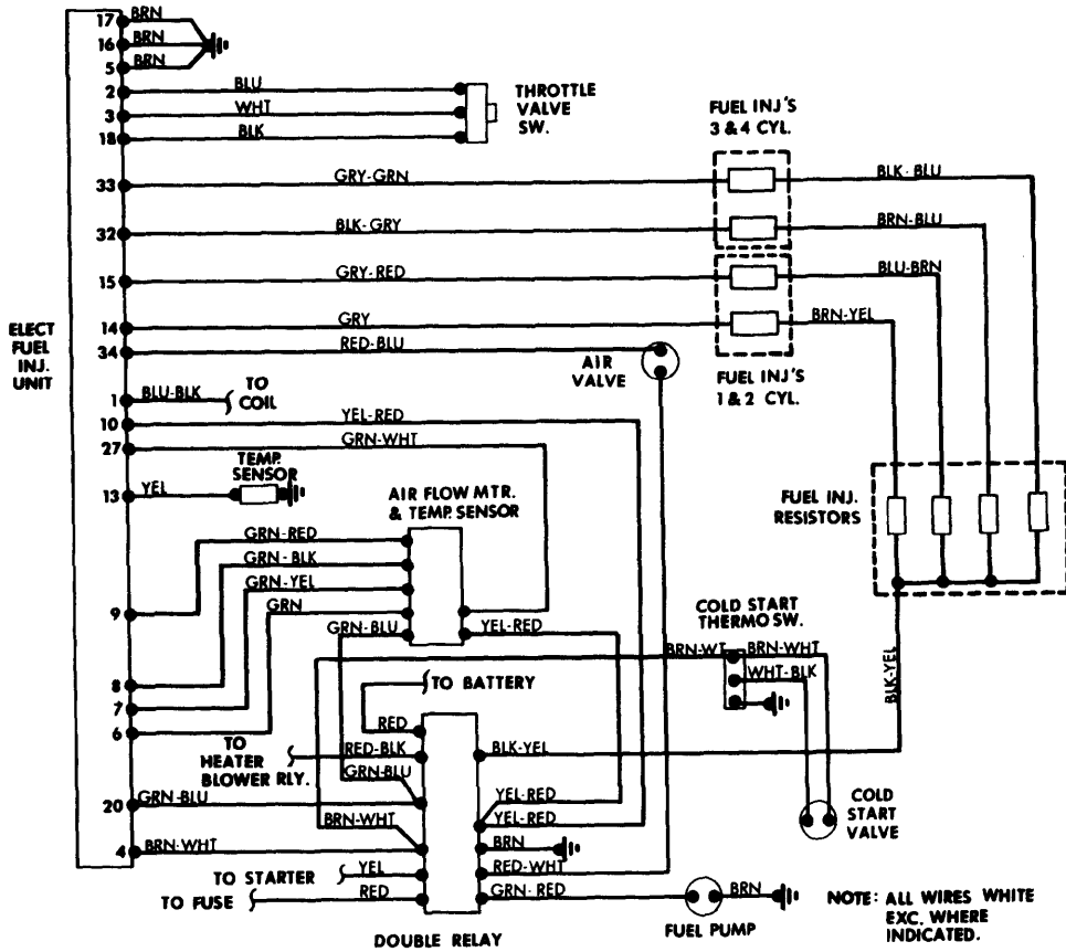
Fuel Injection System Wiring Diagram (Porsche 912E)
