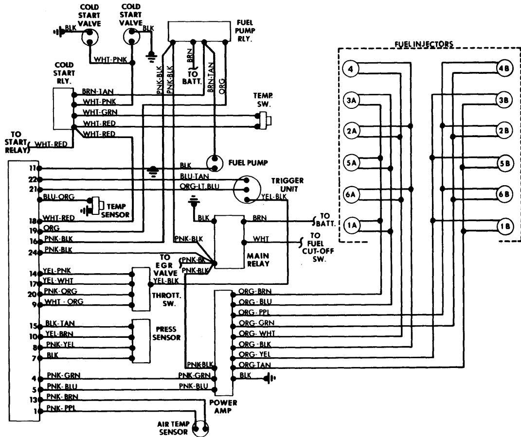
Fuel Injection System Wiring Diagram (Jaguar XJ12 and XJS)
