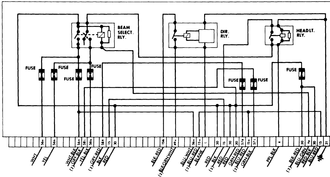
Fuse and Relay Control Box (Audi 100LS)
