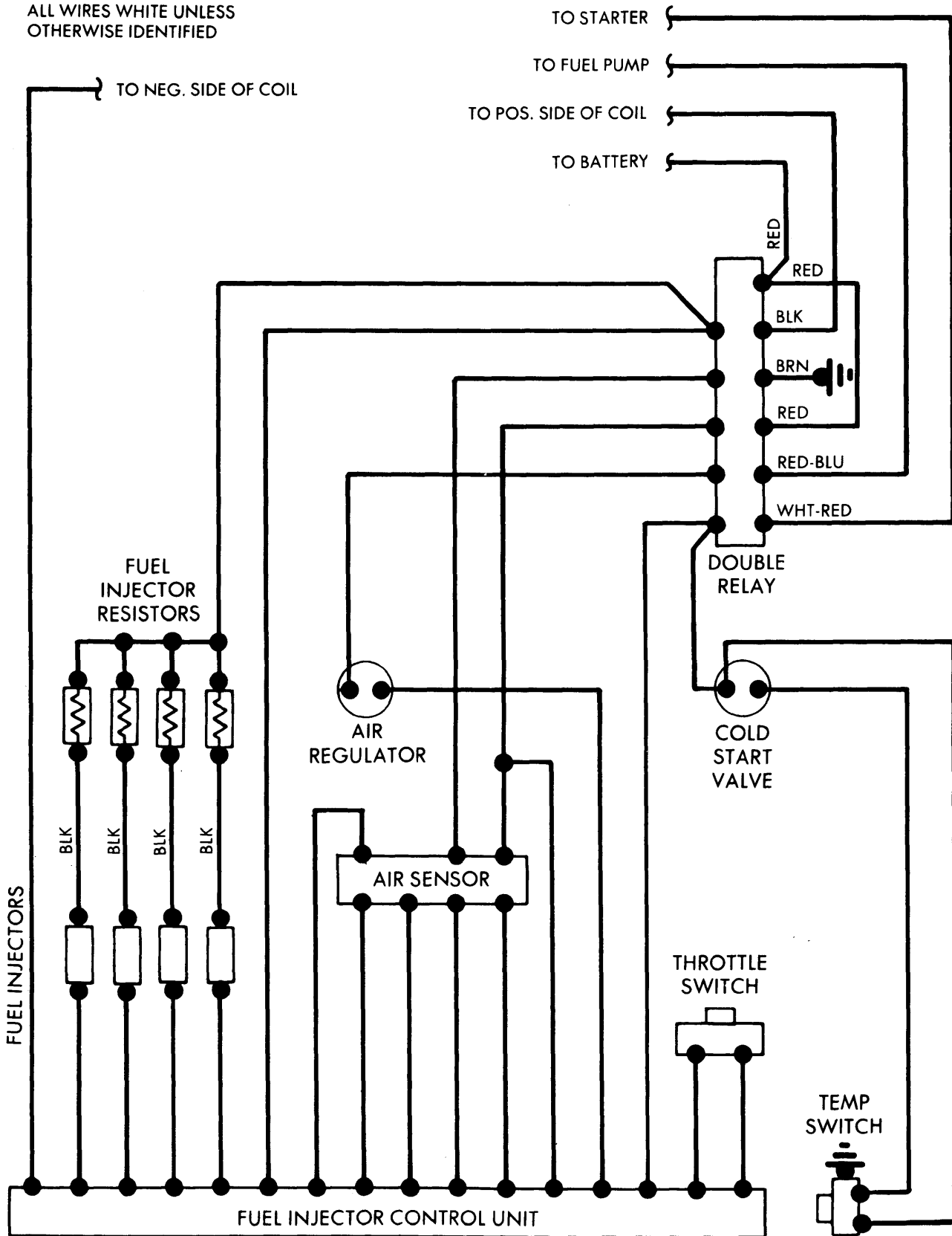
TYPE 1 & 2 BOSCH FUEL INJECTION WIRING DIAGRAM
