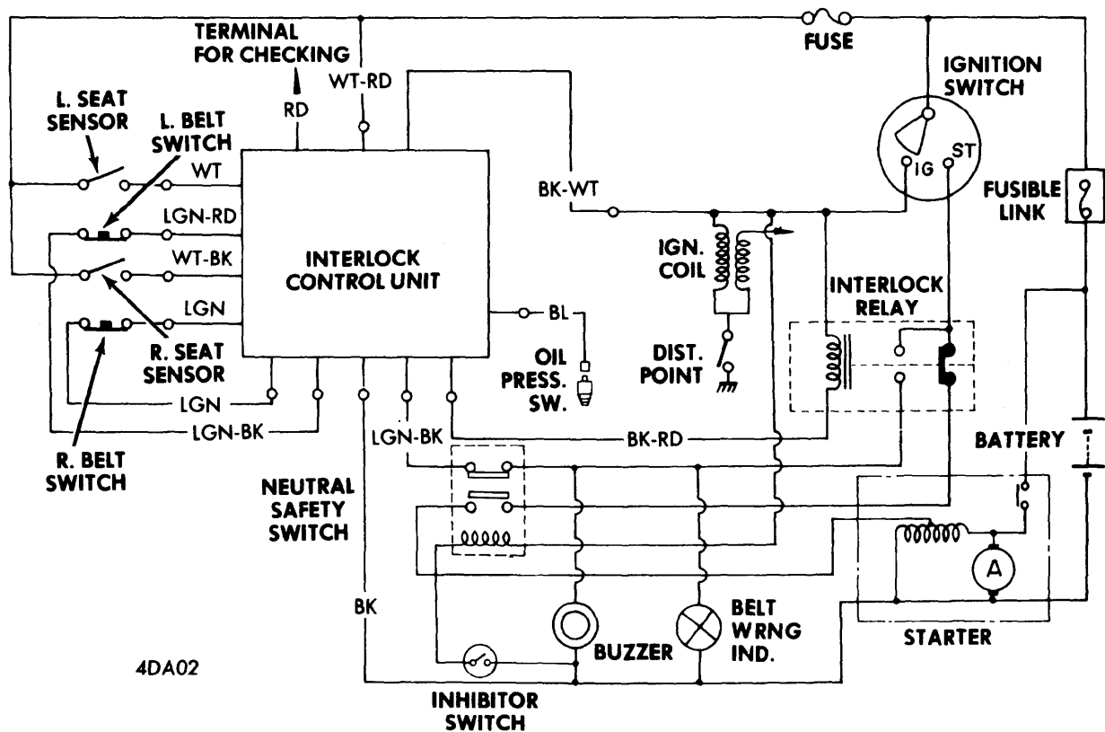
DATSUN 210 (AUTOMATIC TRANSMISSION)
