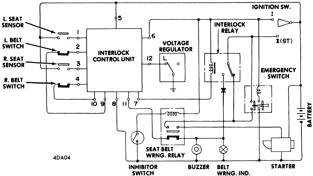
DATSUN 610, 710, 260Z, 620 (MANUAL TRANSMISSION)
