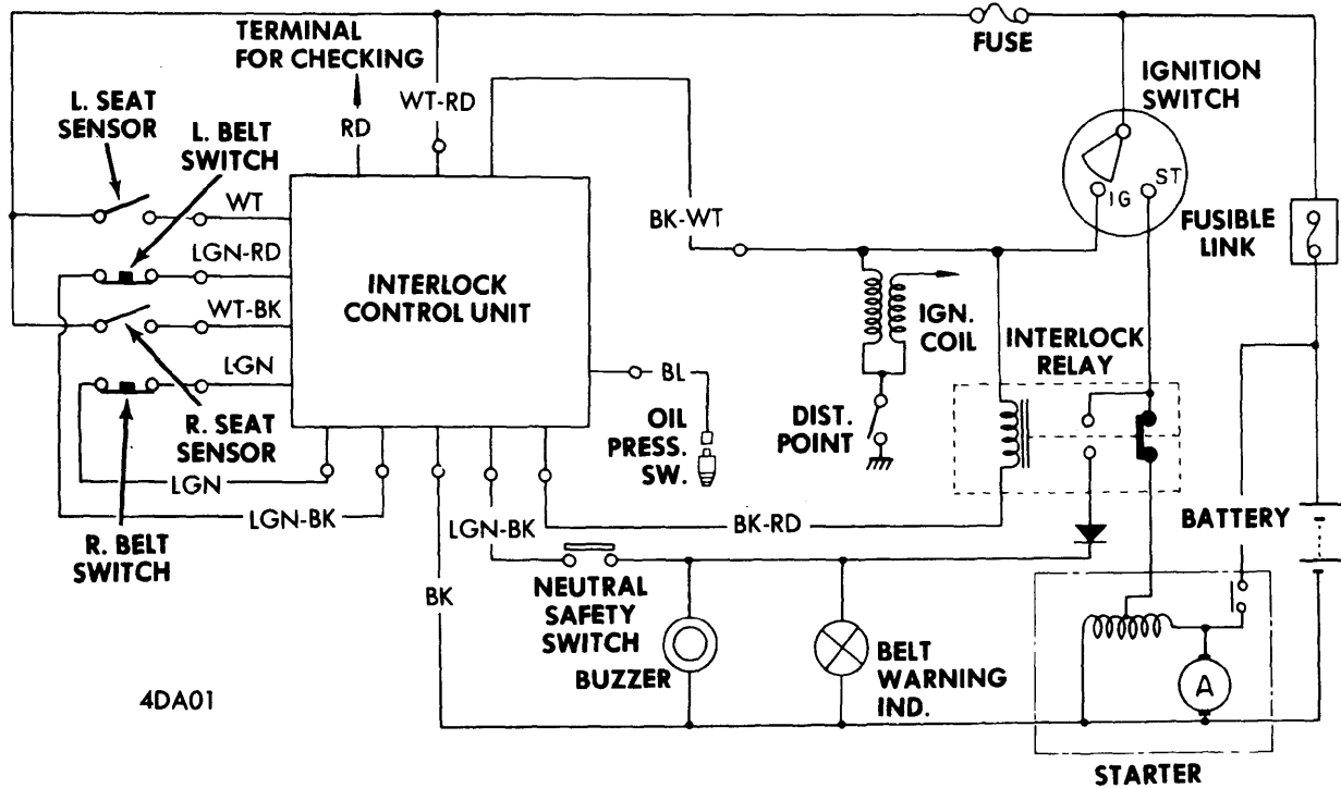
DATSUN 210 (MANUAL TRANSMISSION)
