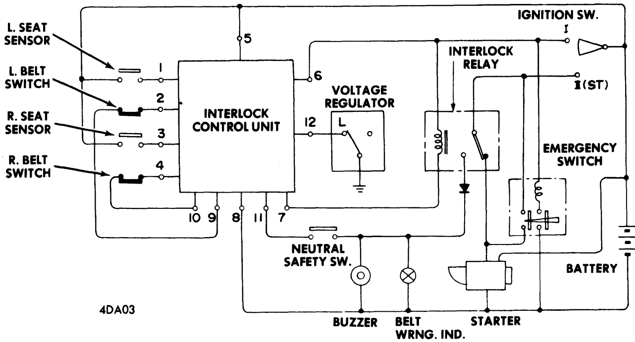
DATSUN 610, 710, 260Z, 620 (AUTOMATIC TRANSMISSION)
