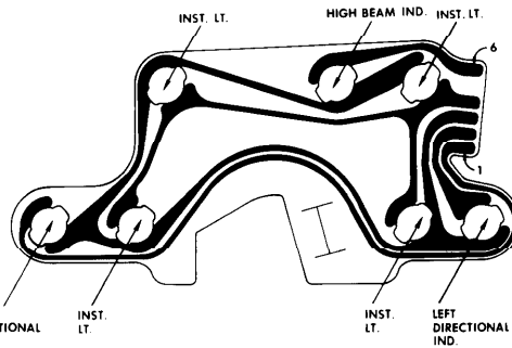
DEVILLE & BROUGHM SPEEDO CLUSTER PRINTED CIRCUIT CONN.
