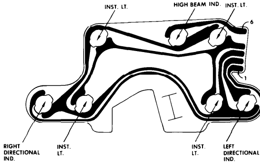
DEVILLE & BROUGHM SPEEDO CLUSTER PRINTED CIRCUIT CONN.
