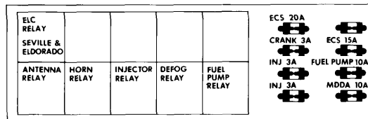
FUSE & RELAY BOX
