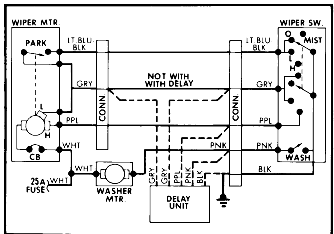
Integral Wiper System Wiring Diagram for General Motors (Citation, Omega, Phoenix, Skylark Standard & Intermittent)
