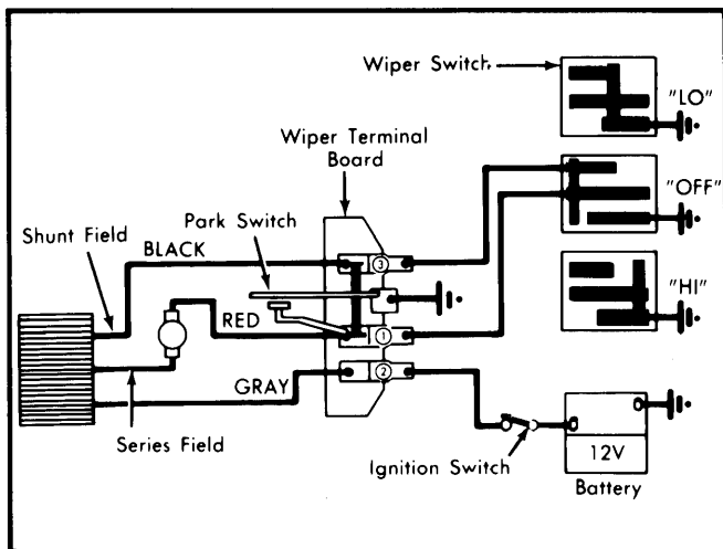
Square Motor Wiper System Wiring Diagram for General Motors
