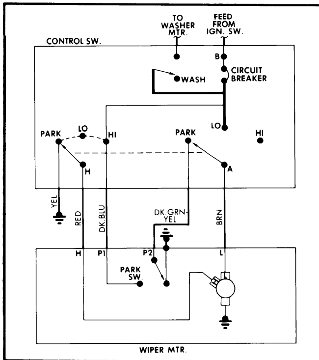
2-Speed Wiper Wiring Diagram for Chrysler Corp. (Aspen, Volare, LeBaron & Diplomat Models)
