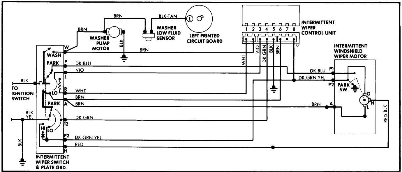
Intermittent Wiper Wiring Diagram for Chrysler Corp.
