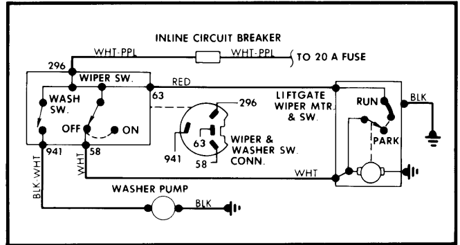
Rear Wiper/Washer System Wiring Diagram for Ford Motor Co.
