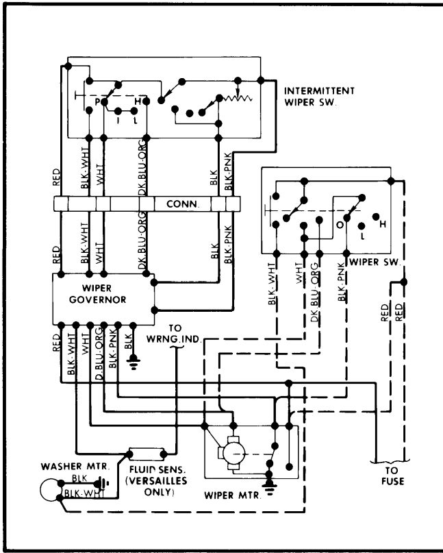
Non-Concealed Wiper System Wiring Diagram for Ford Motor Co. (Granada, Monarch & Versailles)
