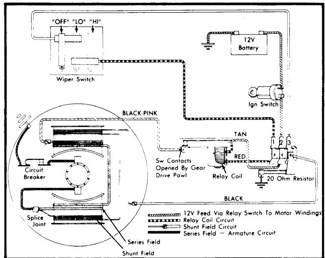
Round Motor Wiper System Diagram for General Motors
