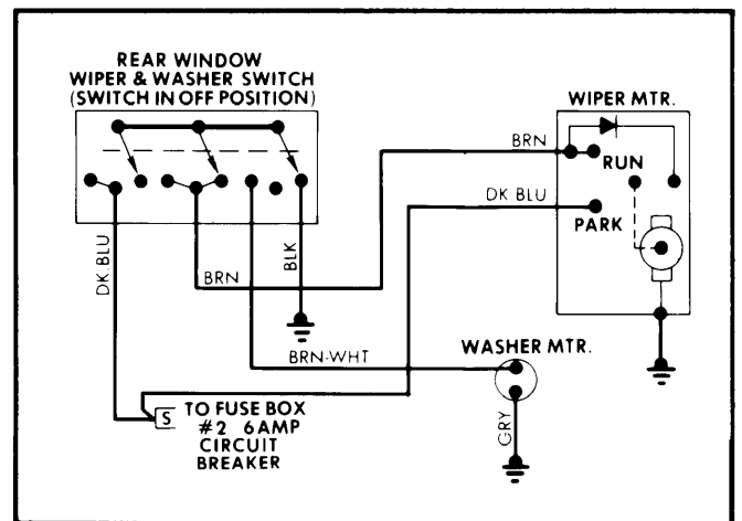
Liftgate Wiper Wiring Diagram for Chrysler Corp. (Omni & Horizon Models)
