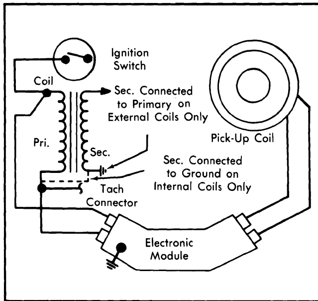
Delco-Remy High Energy Ignition (HEI) System Wiring Diagram for General Motors
