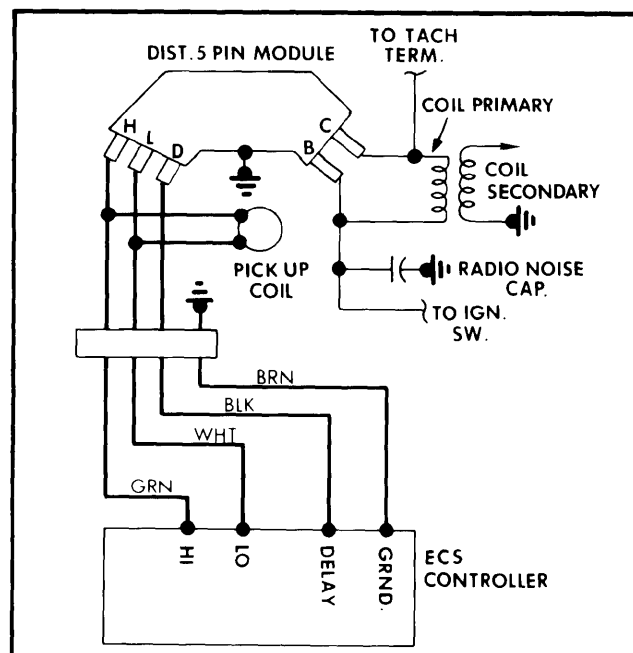
Electronic Spark Control (ESC) Ignition System Wiring Diagram for General Motors (Without Turbocharger)
