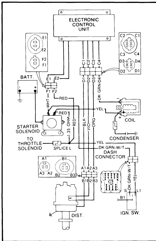
Solid State Ignition System Wiring Diagram for American Motors
