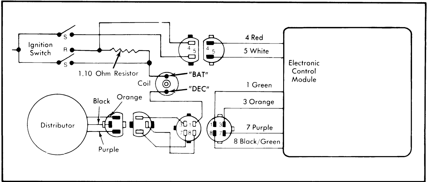
Dura-Spark II Ignition System Wiring Diagram for Ford Motor Co.
