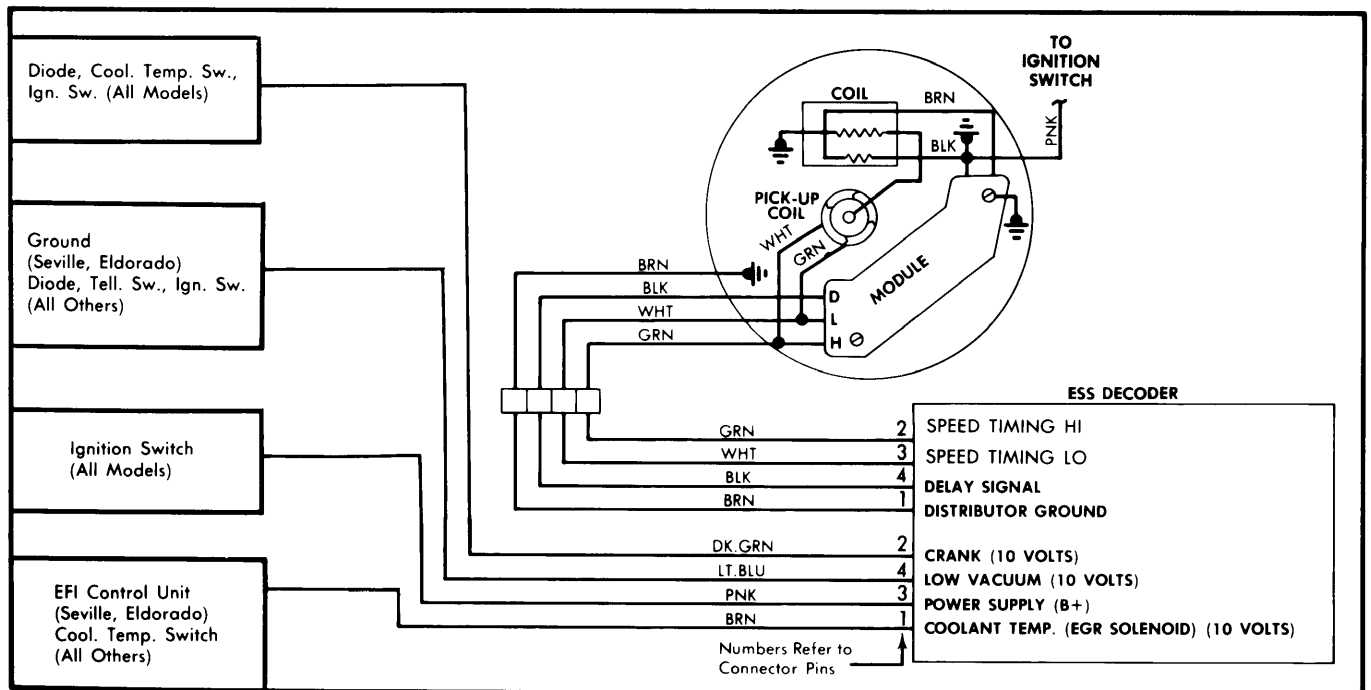
Electronic Spark Selection (ESS) Ignition System Wiring Diagram for General Motors
