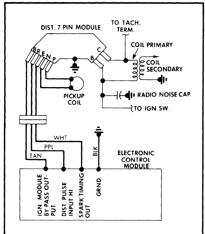
Electronic Spark Timing (EST) Ignition System Wiring Diagram for General Motors
