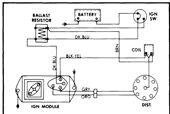
Electronic Ignition Wiring Diagram for Chrysler Corp. (6-Cylinder & V8 Models)
