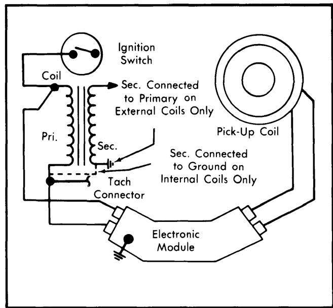
Delco-Remy High Energy Ignition (HEI) System Wiring Diagram for American Motors (4-Cylinder Models Only)
