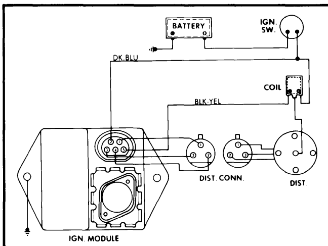
Electronic Ignition Wiring Diagram for Chrysler Corp. (4-Cylinder Models)
