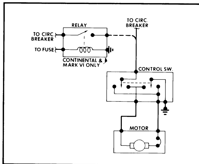
Power Roof Panel Wiring Diagram for Ford Motor Co.
