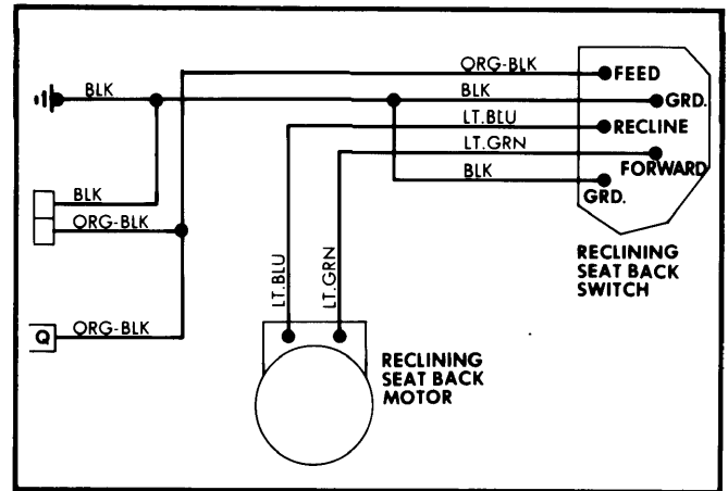
Power Reclining Seat Back Wiring Diagram for General Motors
