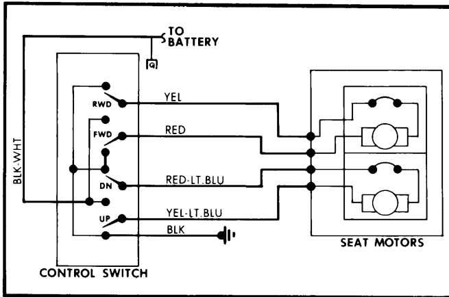
4-Way Power Seat Wiring Diagram for Ford Motor Co.
