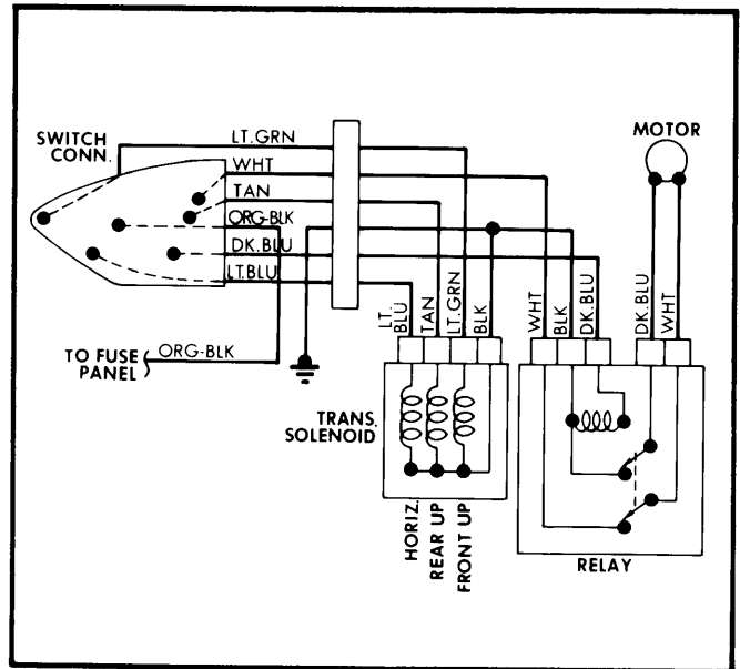
6-Way Power Seat Wiring Diagram for General Motors (Single Motor)
