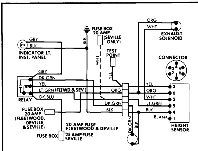
Electronic Level Control Wiring Diagram for Cadillac (Exc. Eldorado and Seville)
