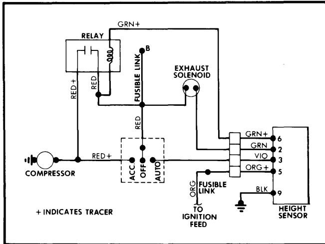
Electronic Level Control Wiring Diagram for American Motors
