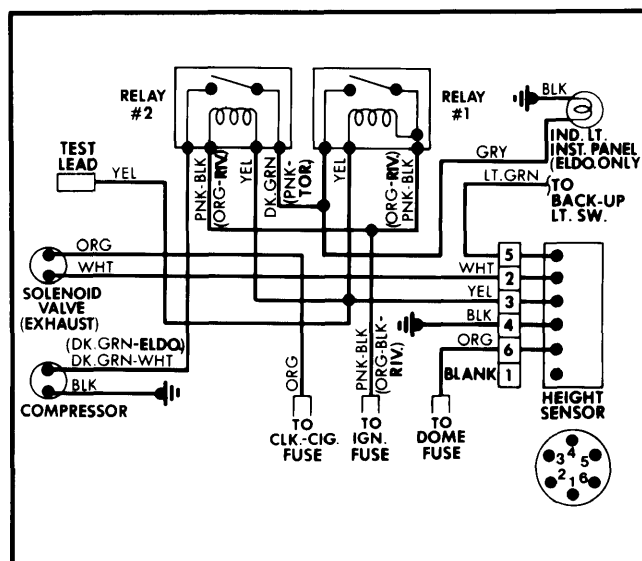
Electronic Level Control Wiring Diagram for Eldorado, Riviera, Seville and Toronado
