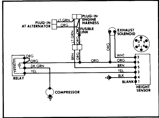
Electronic Level Control Wiring Diagram for Buick (Exc. Riviera) and Pontiac
