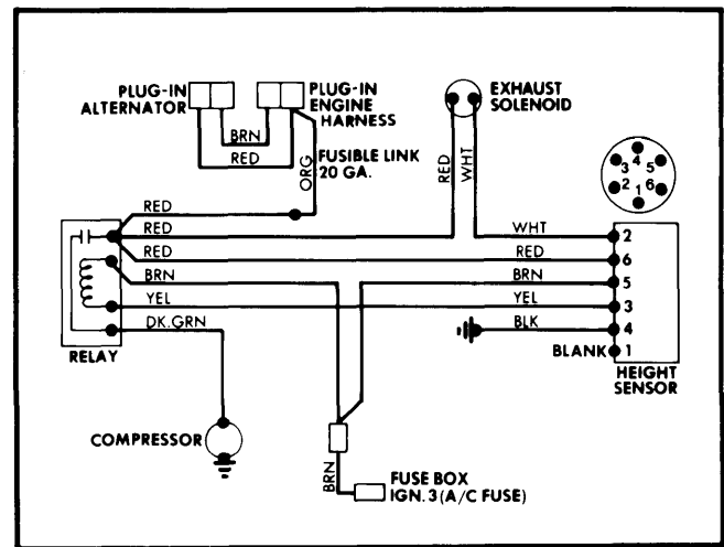
Electronic Level Control Wiring Diagram for Oldsmobile (Exc. Toronado)
